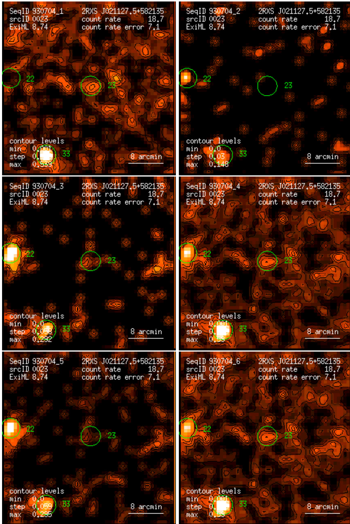
Figure 23: RASS 930704: detection 0023: band rate images, Gaussian filter: (1) PSPC channels 11 – 41, (2) 52 – 90, (3) 91 – 201, (4) 11 – 235, (5) 52 – 201, (6) 11 – 201. Broad band rates in counts/ks. Band rate contour levels in counts/ks/arcmin 2 .
