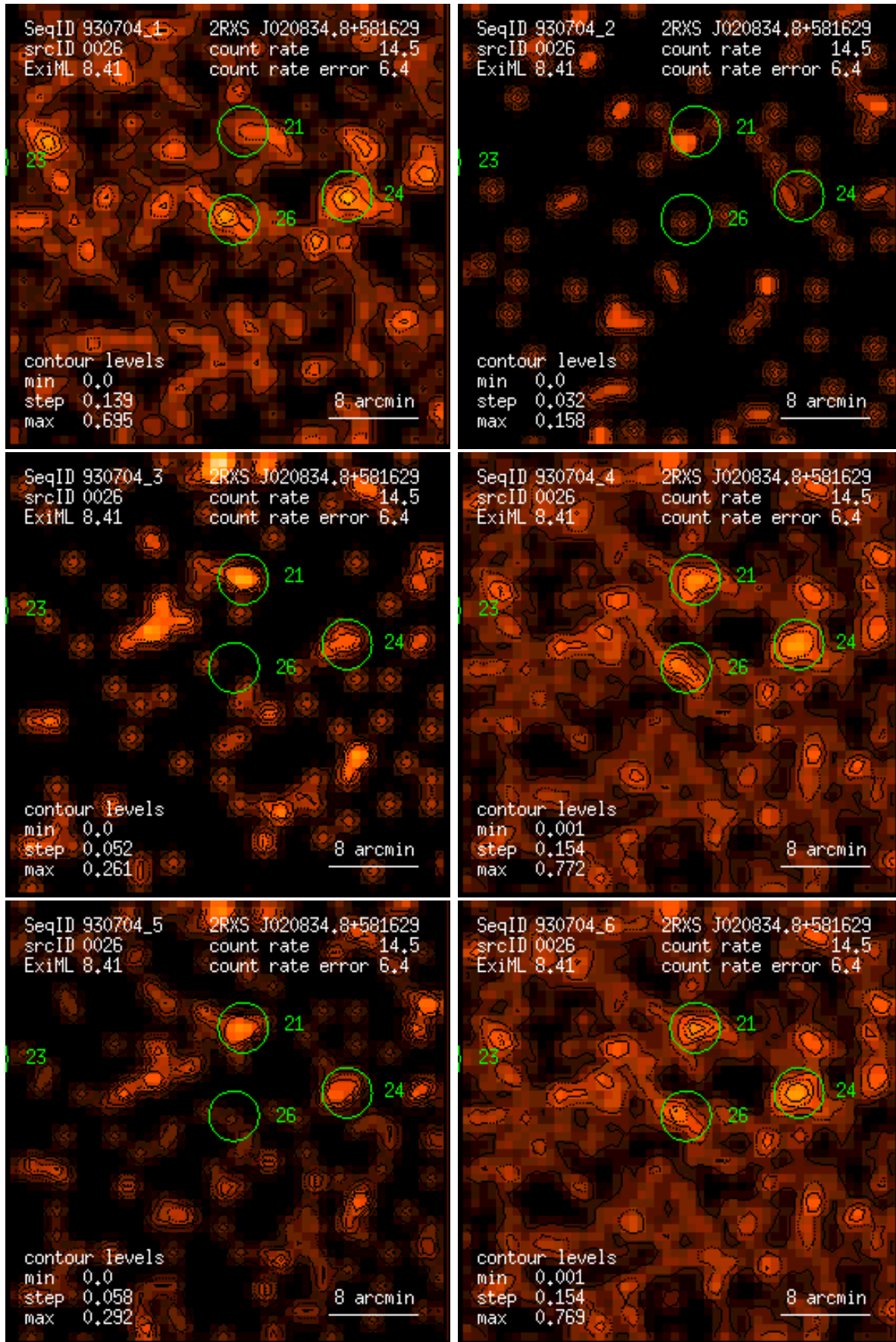
Figure 26: RASS 930704: detection 0026: band rate images, Gaussian filter: (1) PSPC channels 11 – 41, (2) 52 – 90, (3) 91 – 201, (4) 11 – 235, (5) 52 – 201, (6) 11 – 201. Broad band rates in counts/ks. Band rate contour levels in counts/ks/arcmin 2 .
