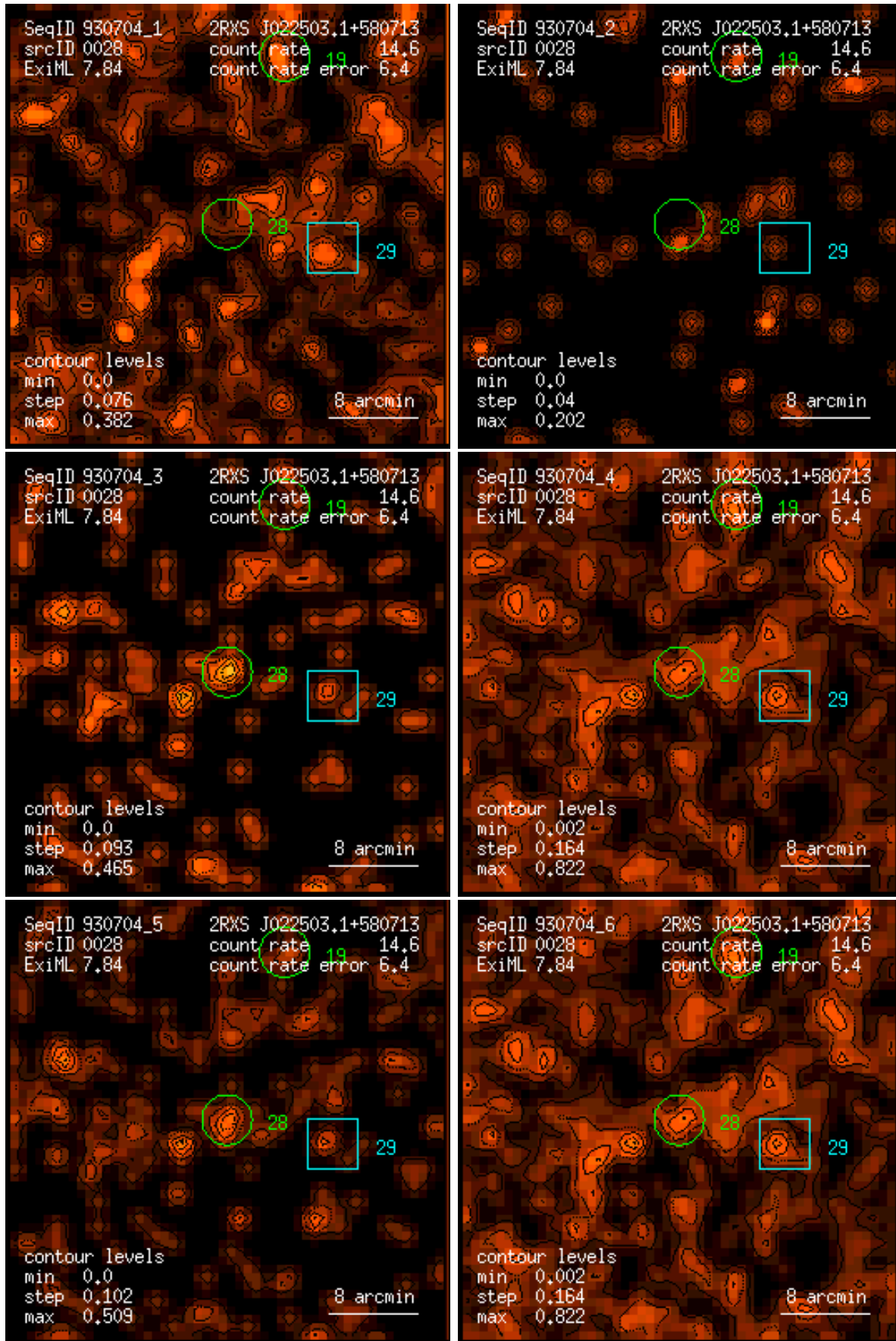
Figure 28: RASS 930704: detection 0028: band rate images, Gaussian filter: (1) PSPC channels 11 – 41, (2) 52 – 90, (3) 91 – 201, (4) 11 – 235, (5) 52 – 201, (6) 11 – 201. Broad band rates in counts/ks. Band rate contour levels in counts/ks/arcmin 2 .
