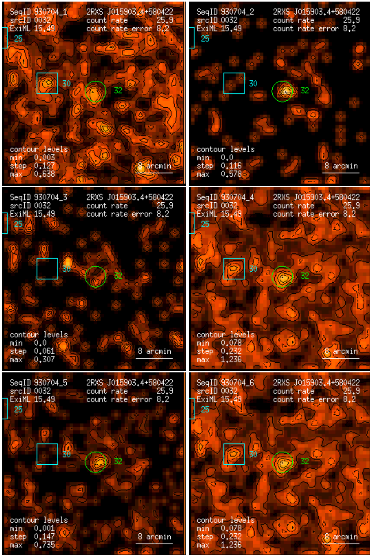
Figure 32: RASS 930704: detection 0032: band rate images, Gaussian filter: (1) PSPC channels 11 – 41, (2) 52 – 90, (3) 91 – 201, (4) 11 – 235, (5) 52 – 201, (6) 11 – 201. Broad band rates in counts/ks. Band rate contour levels in counts/ks/arcmin 2 .
