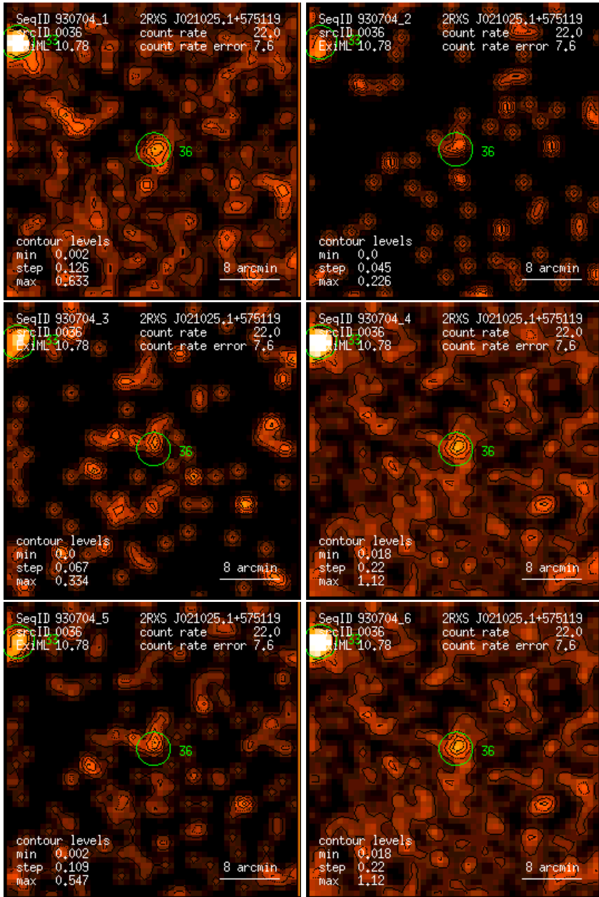
Figure 36: RASS 930704: detection 0036: band rate images, Gaussian filter: (1) PSPC channels 11 – 41, (2) 52 – 90, (3) 91 – 201, (4) 11 – 235, (5) 52 – 201, (6) 11 – 201. Broad band rates in counts/ks. Band rate contour levels in counts/ks/arcmin 2 .
