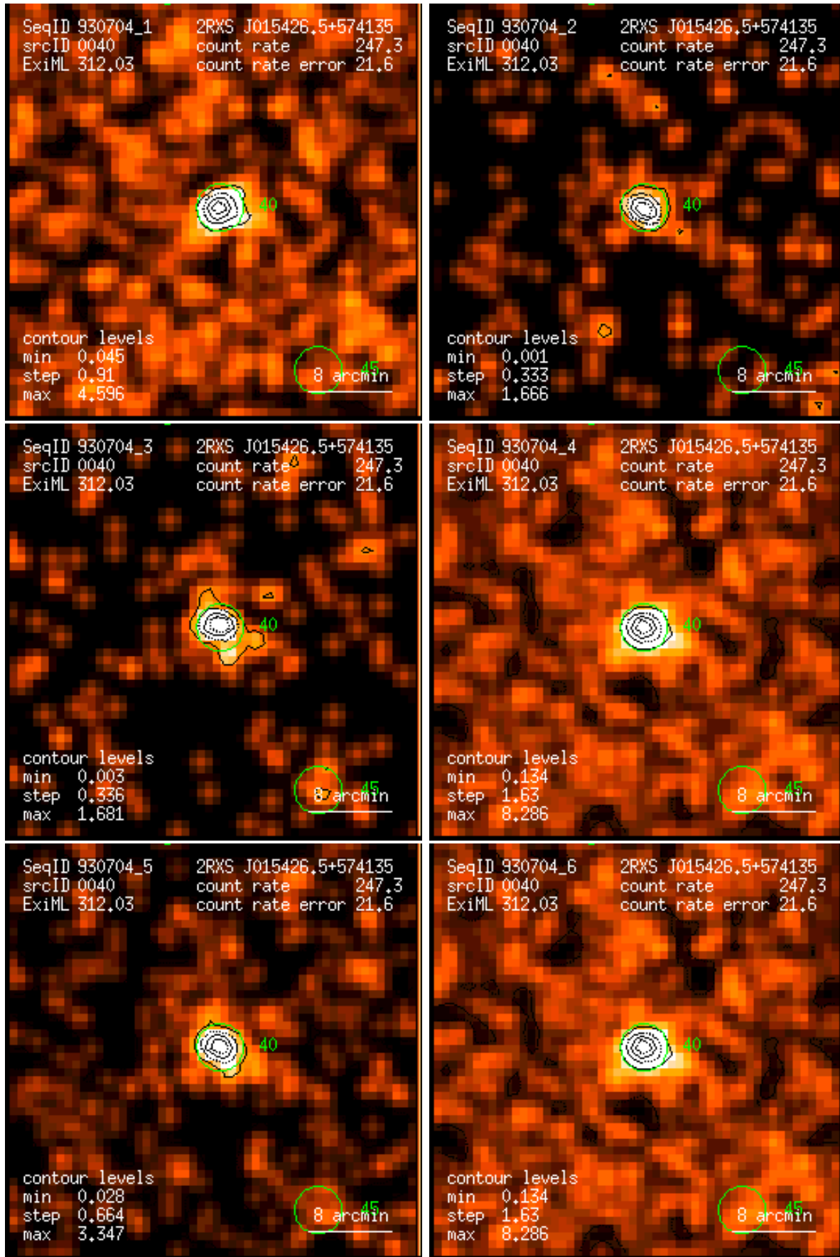
Figure 40: RASS 930704: detection 0040: band rate images, Gaussian filter: (1) PSPC channels 11 – 41, (2) 52 – 90, (3) 91 – 201, (4) 11 – 235, (5) 52 – 201, (6) 11 – 201. Broad band rates in counts/ks. Band rate contour levels in counts/ks/arcmin 2 .
