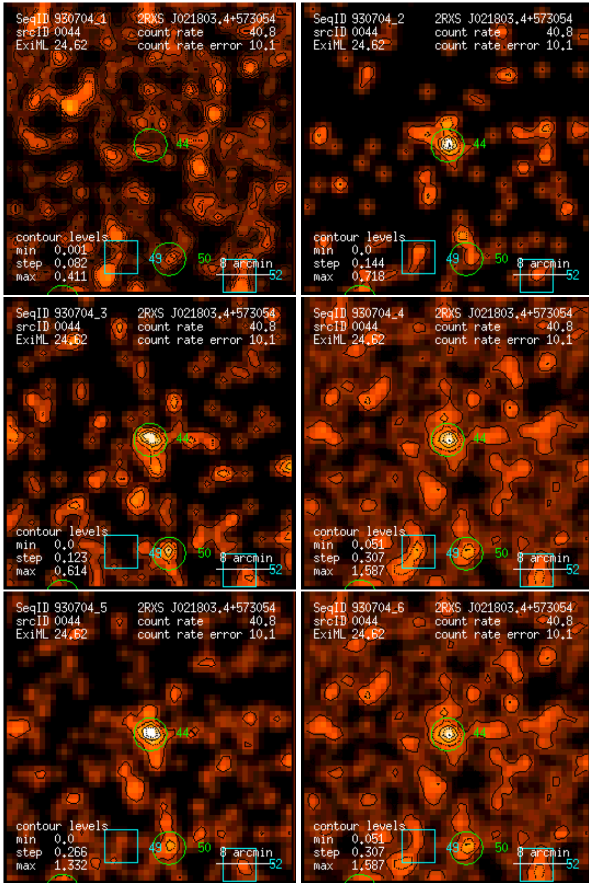
Figure 44: RASS 930704: detection 0044: band rate images, Gaussian filter: (1) PSPC channels 11 – 41, (2) 52 – 90, (3) 91 – 201, (4) 11 – 235, (5) 52 – 201, (6) 11 – 201. Broad band rates in counts/ks. Band rate contour levels in counts/ks/arcmin 2 .
