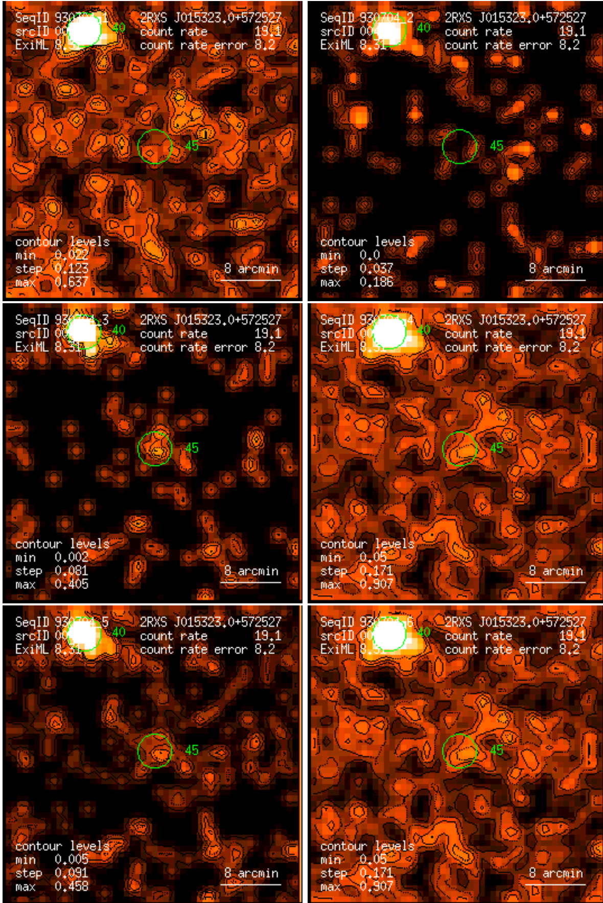
Figure 45: RASS 930704: detection 0045: band rate images, Gaussian filter: (1) PSPC channels 11 – 41, (2) 52 – 90, (3) 91 – 201, (4) 11 – 235, (5) 52 – 201, (6) 11 – 201. Broad band rates in counts/ks. Band rate contour levels in counts/ks/arcmin 2 .
