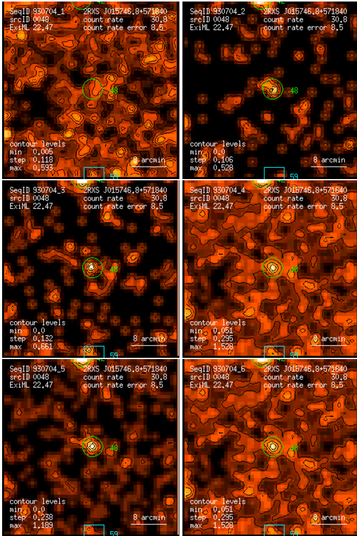
Figure 48: RASS 930704: detection 0048: band rate images, Gaussian filter: (1) PSPC channels 11 – 41, (2) 52 – 90, (3) 91 – 201, (4) 11 – 235, (5) 52 – 201, (6) 11 – 201. Broad band rates in counts/ks. Band rate contour levels in counts/ks/arcmin 2 .
