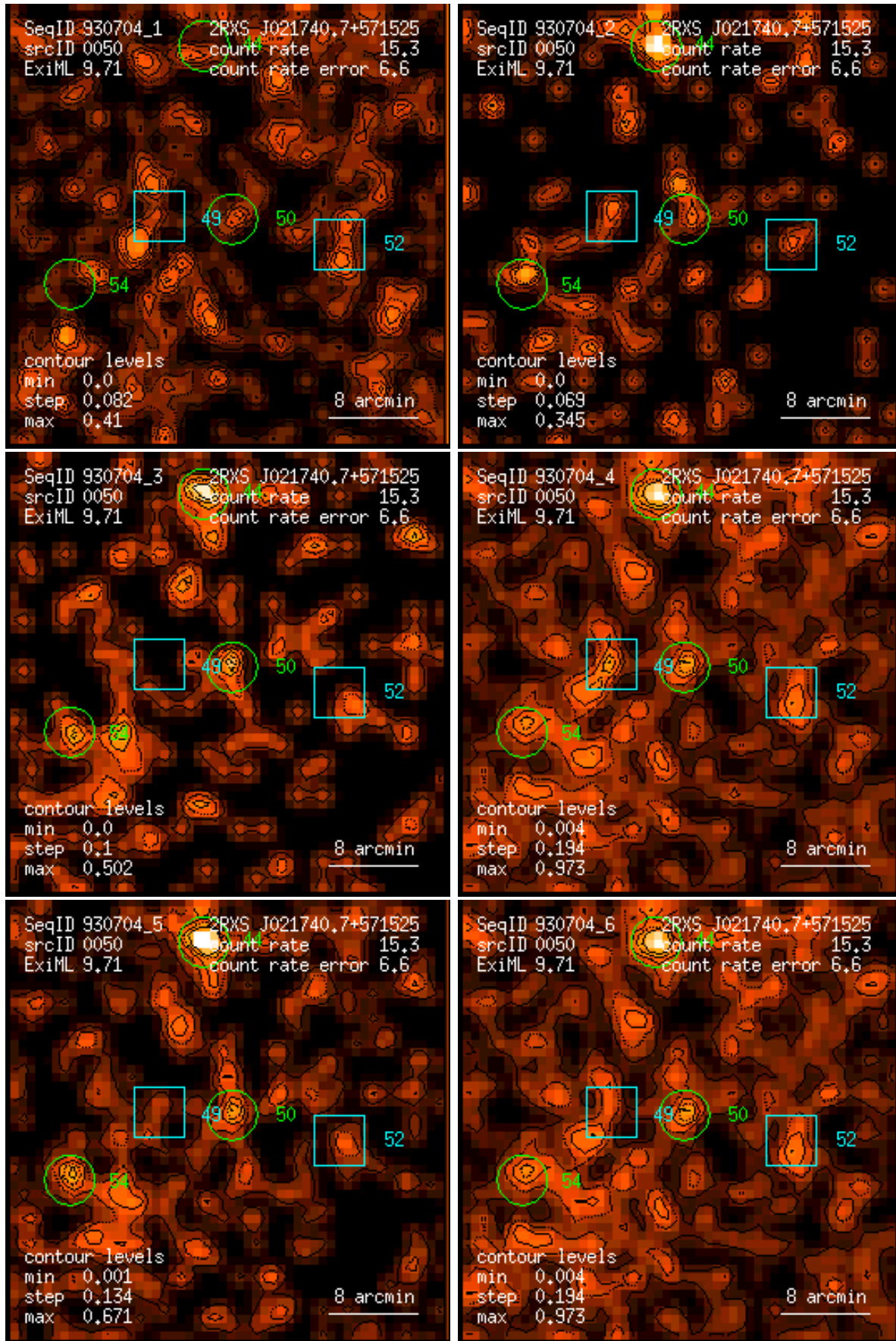
Figure 50: RASS 930704: detection 0050: band rate images, Gaussian filter: (1) PSPC channels 11 – 41, (2) 52 – 90, (3) 91 – 201, (4) 11 – 235, (5) 52 – 201, (6) 11 – 201. Broad band rates in counts/ks. Band rate contour levels in counts/ks/arcmin 2 .
