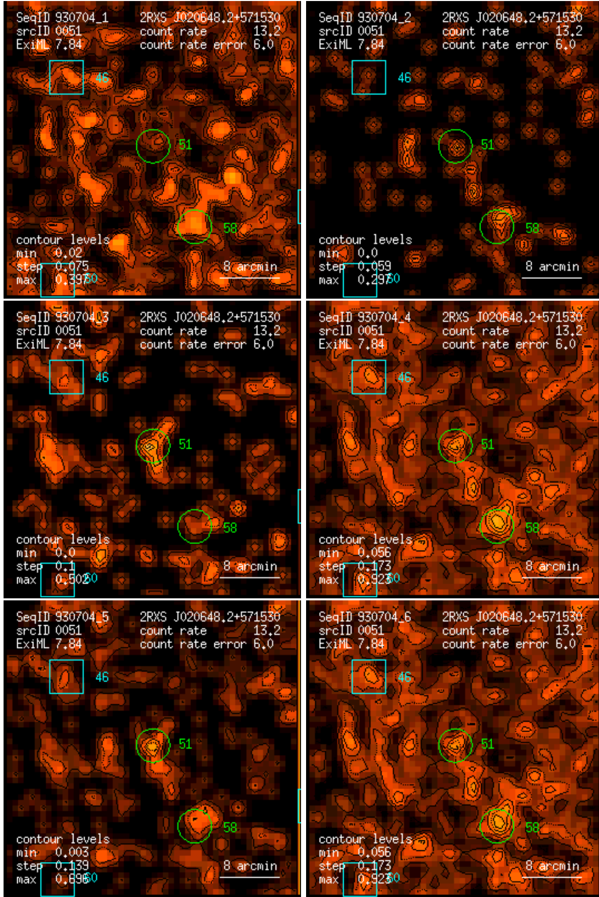
Figure 51: RASS 930704: detection 0051: band rate images, Gaussian filter: (1) PSPC channels 11 – 41, (2) 52 – 90, (3) 91 – 201, (4) 11 – 235, (5) 52 – 201, (6) 11 – 201. Broad band rates in counts/ks. Band rate contour levels in counts/ks/arcmin 2 .
