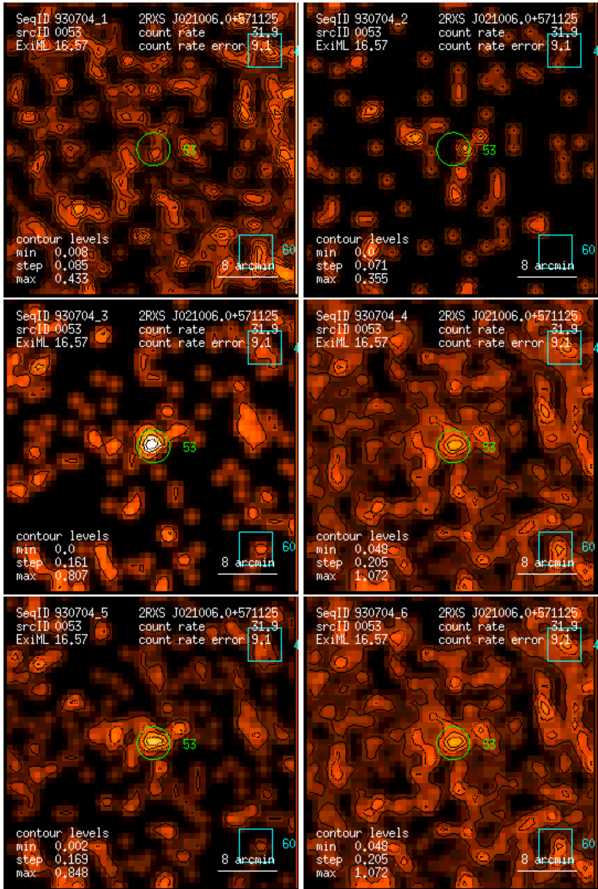
Figure 53: RASS 930704: detection 0053: band rate images, Gaussian filter: (1) PSPC channels 11 – 41, (2) 52 – 90, (3) 91 – 201, (4) 11 – 235, (5) 52 – 201, (6) 11 – 201. Broad band rates in counts/ks. Band rate contour levels in counts/ks/arcmin 2 .
