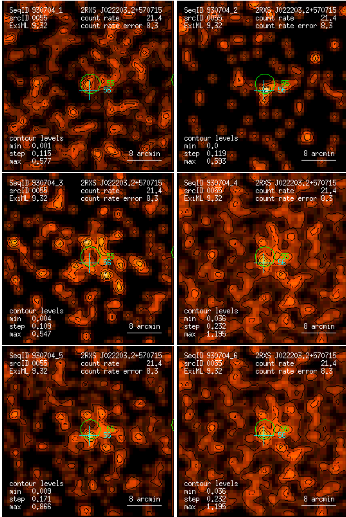
Figure 55: RASS 930704: detection 0055: band rate images, Gaussian filter: (1) PSPC channels 11 – 41, (2) 52 – 90, (3) 91 – 201, (4) 11 – 235, (5) 52 – 201, (6) 11 – 201. Broad band rates in counts/ks. Band rate contour levels in counts/ks/arcmin 2 .
