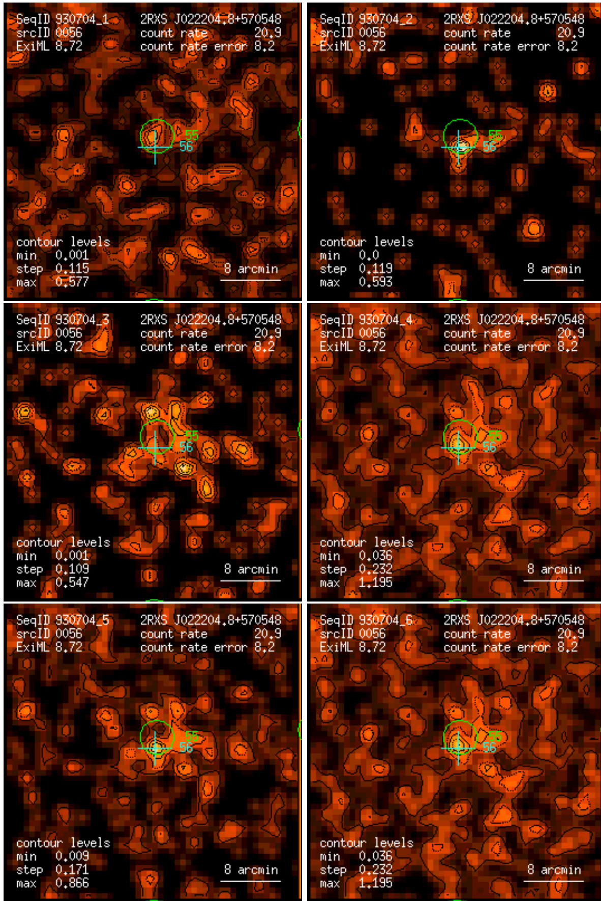
Figure 56: RASS 930704: detection 0056: band rate images, Gaussian filter: (1) PSPC channels 11 – 41, (2) 52 – 90, (3) 91 – 201, (4) 11 – 235, (5) 52 – 201, (6) 11 – 201. Broad band rates in counts/ks. Band rate contour levels in counts/ks/arcmin 2 .
