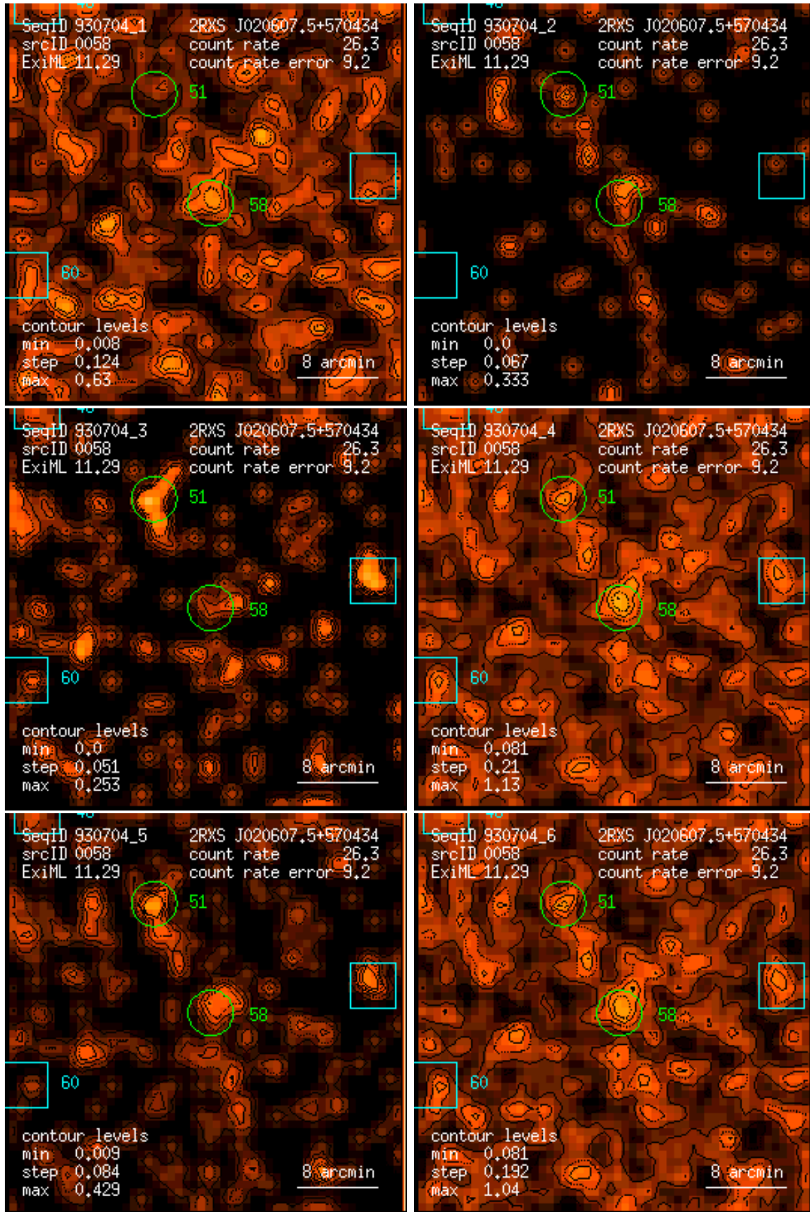
Figure 58: RASS 930704: detection 0058: band rate images, Gaussian filter: (1) PSPC channels 11 – 41, (2) 52 – 90, (3) 91 – 201, (4) 11 – 235, (5) 52 – 201, (6) 11 – 201. Broad band rates in counts/ks. Band rate contour levels in counts/ks/arcmin 2 .
