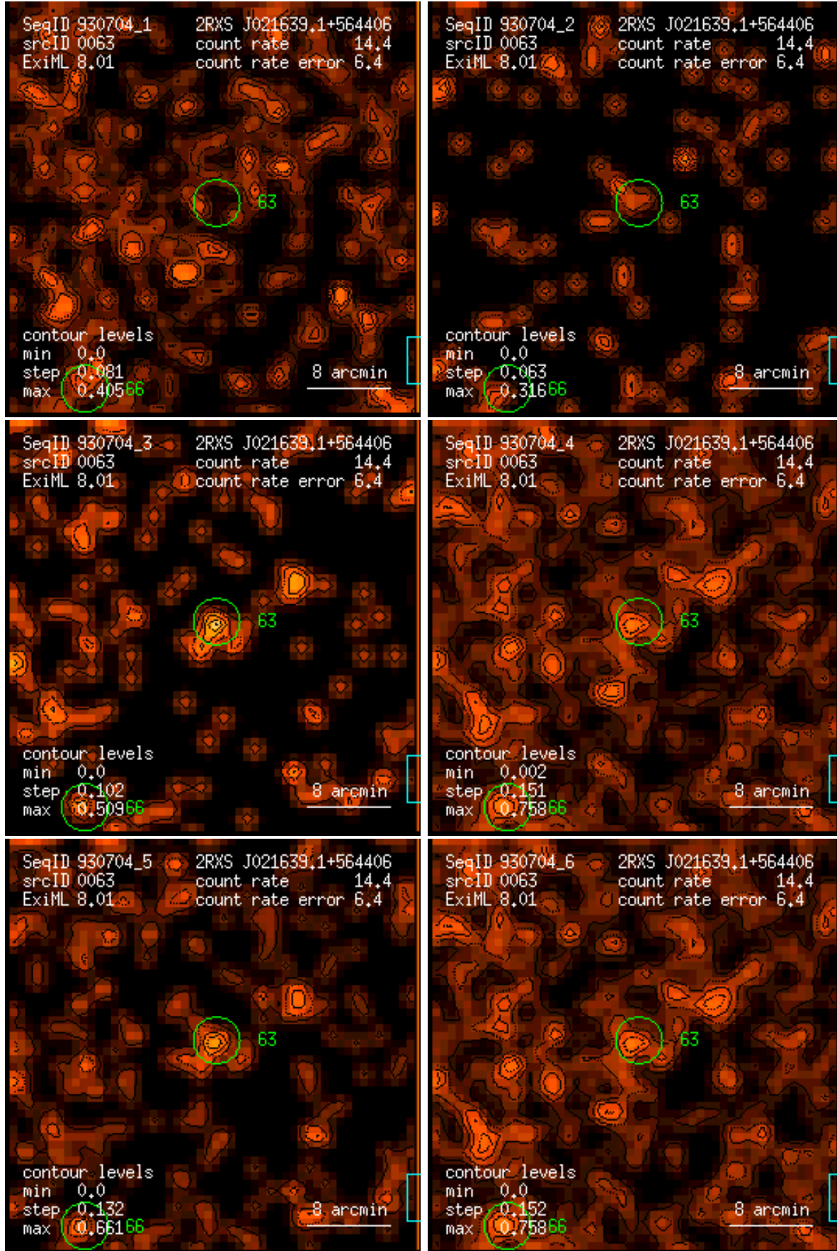
Figure 63: RASS 930704: detection 0063: band rate images, Gaussian filter: (1) PSPC channels 11 – 41, (2) 52 – 90, (3) 91 – 201, (4) 11 – 235, (5) 52 – 201, (6) 11 – 201. Broad band rates in counts/ks. Band rate contour levels in counts/ks/arcmin 2 .
