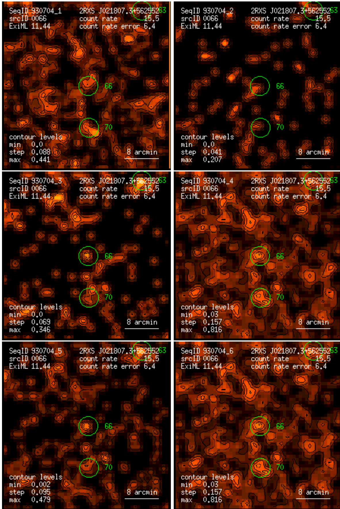
Figure 66: RASS 930704: detection 0066: band rate images, Gaussian filter: (1) PSPC channels 11 – 41, (2) 52 – 90, (3) 91 – 201, (4) 11 – 235, (5) 52 – 201, (6) 11 – 201. Broad band rates in counts/ks. Band rate contour levels in counts/ks/arcmin 2 .
