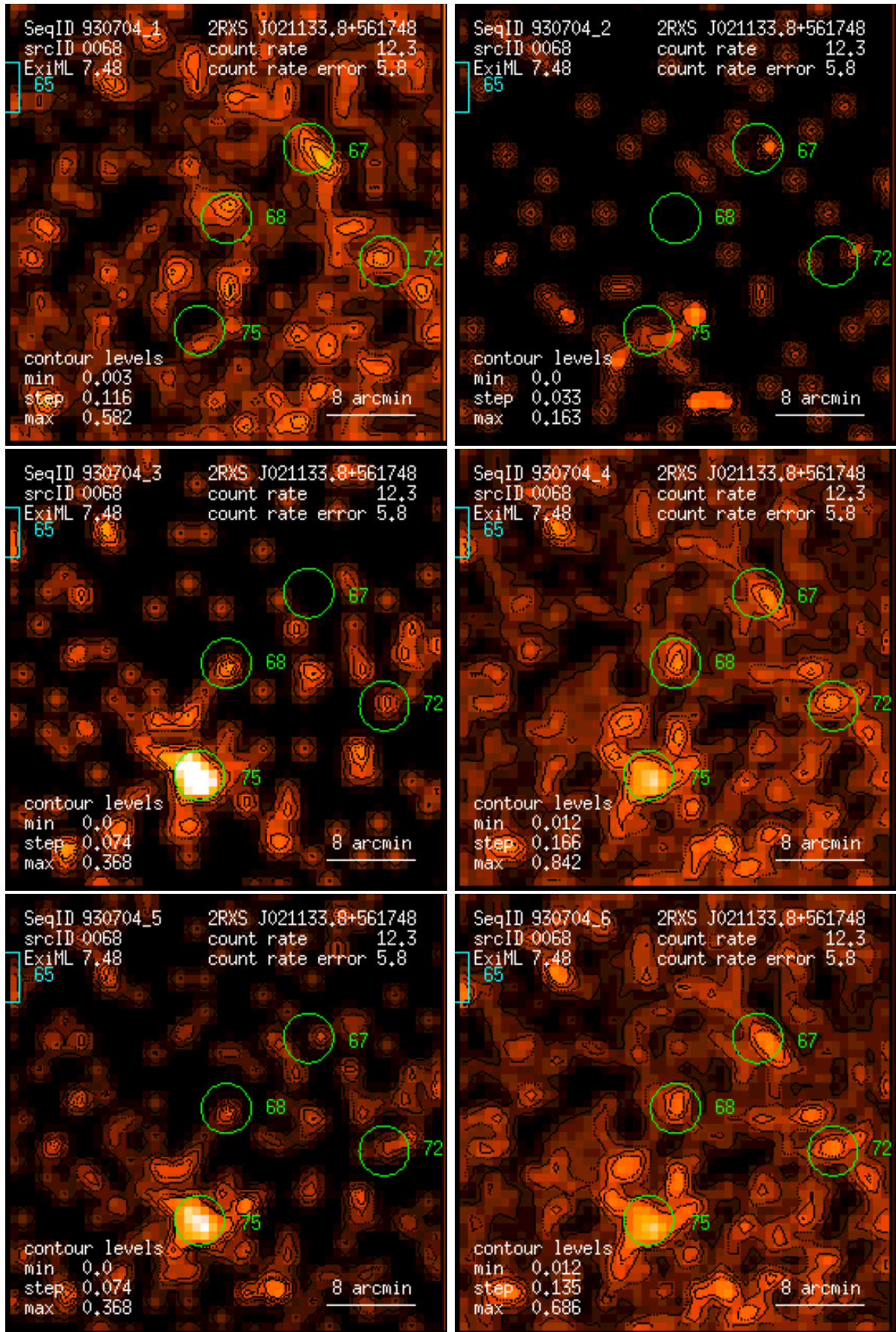
Figure 68: RASS 930704: detection 0068: band rate images, Gaussian filter: (1) PSPC channels 11 – 41, (2) 52 – 90, (3) 91 – 201, (4) 11 – 235, (5) 52 – 201, (6) 11 – 201. Broad band rates in counts/ks. Band rate contour levels in counts/ks/arcmin 2 .
