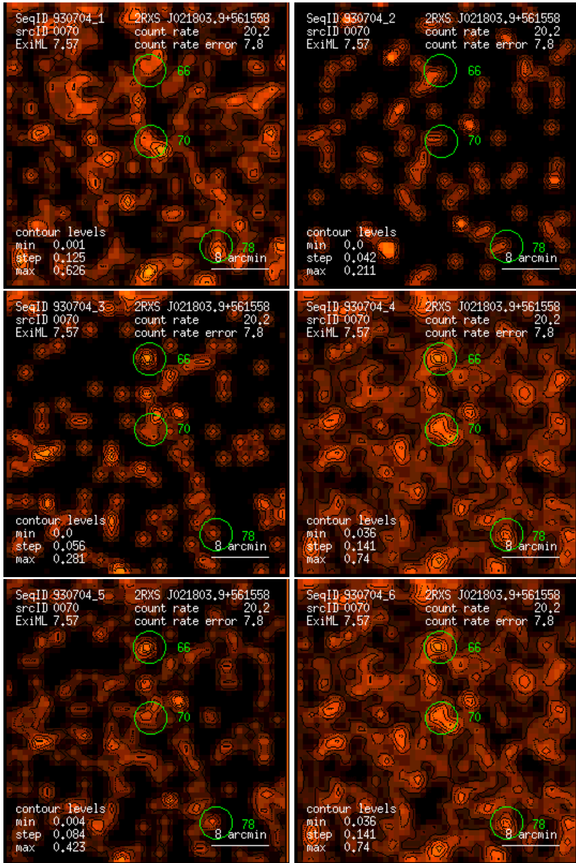
Figure 70: RASS 930704: detection 0070: band rate images, Gaussian filter: (1) PSPC channels 11 – 41, (2) 52 – 90, (3) 91 – 201, (4) 11 – 235, (5) 52 – 201, (6) 11 – 201. Broad band rates in counts/ks. Band rate contour levels in counts/ks/arcmin 2 .
