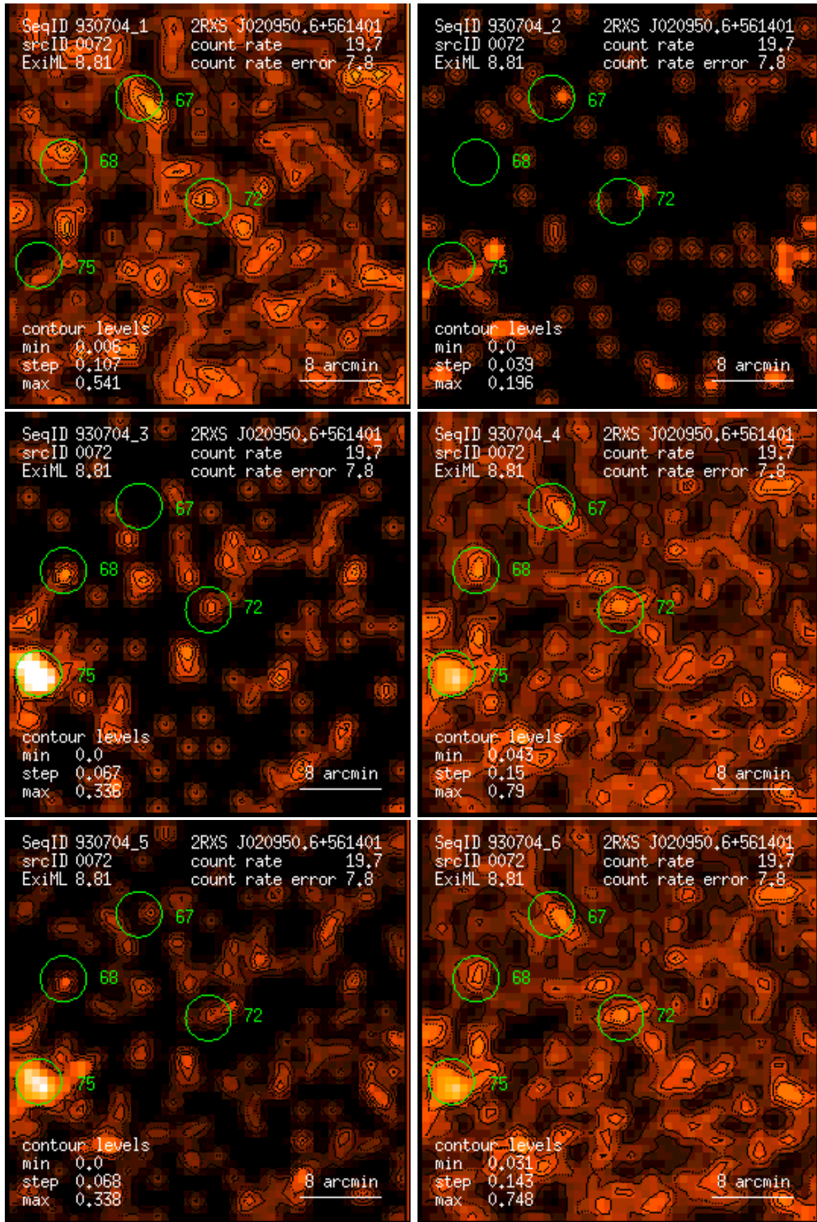
Figure 72: RASS 930704: detection 0072: band rate images, Gaussian filter: (1) PSPC channels 11 – 41, (2) 52 – 90, (3) 91 – 201, (4) 11 – 235, (5) 52 – 201, (6) 11 – 201. Broad band rates in counts/ks. Band rate contour levels in counts/ks/arcmin 2 .
