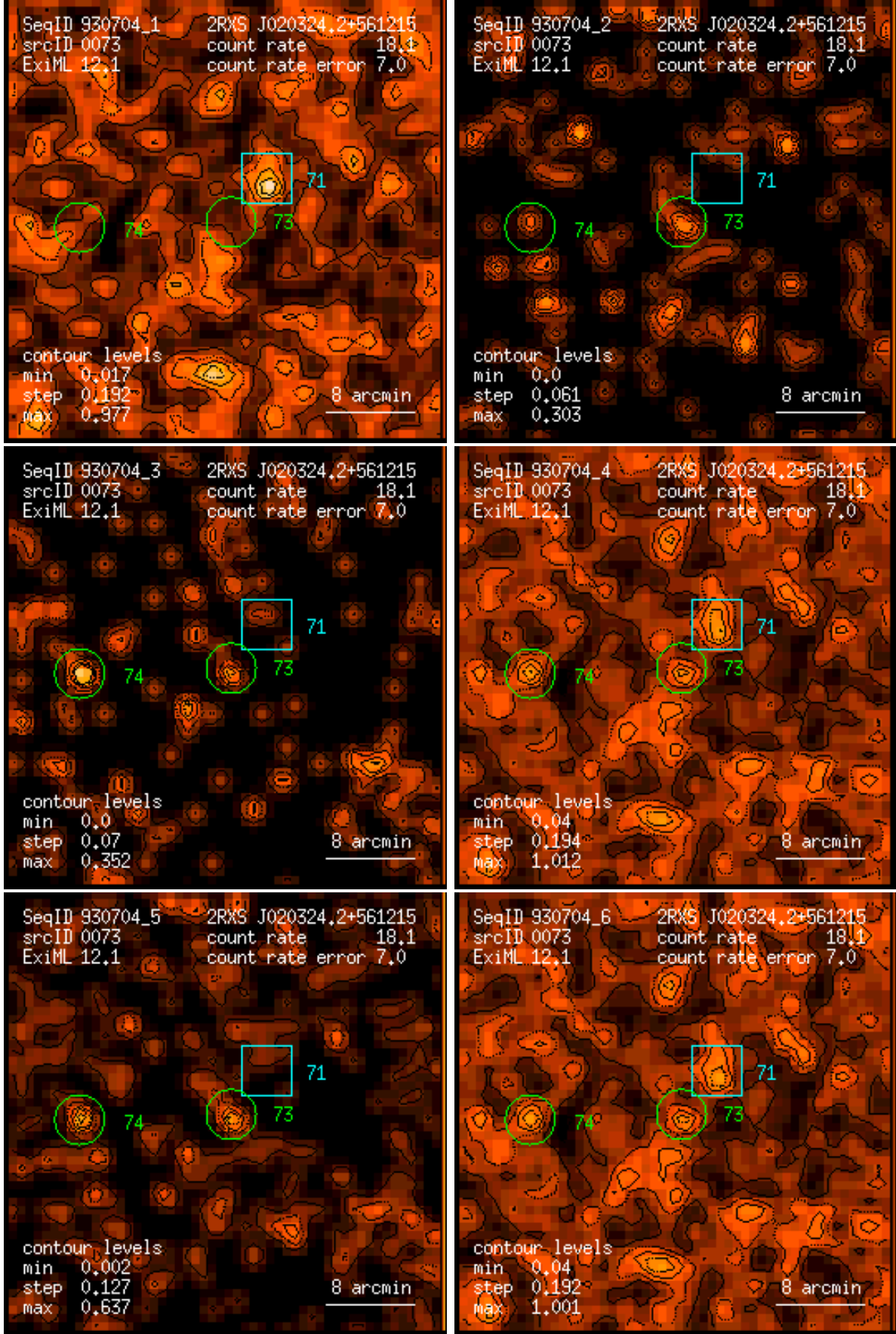
Figure 73: RASS 930704: detection 0073: band rate images, Gaussian filter: (1) PSPC channels 11 – 41, (2) 52 – 90, (3) 91 – 201, (4) 11 – 235, (5) 52 – 201, (6) 11 – 201. Broad band rates in counts/ks. Band rate contour levels in counts/ks/arcmin 2 .
