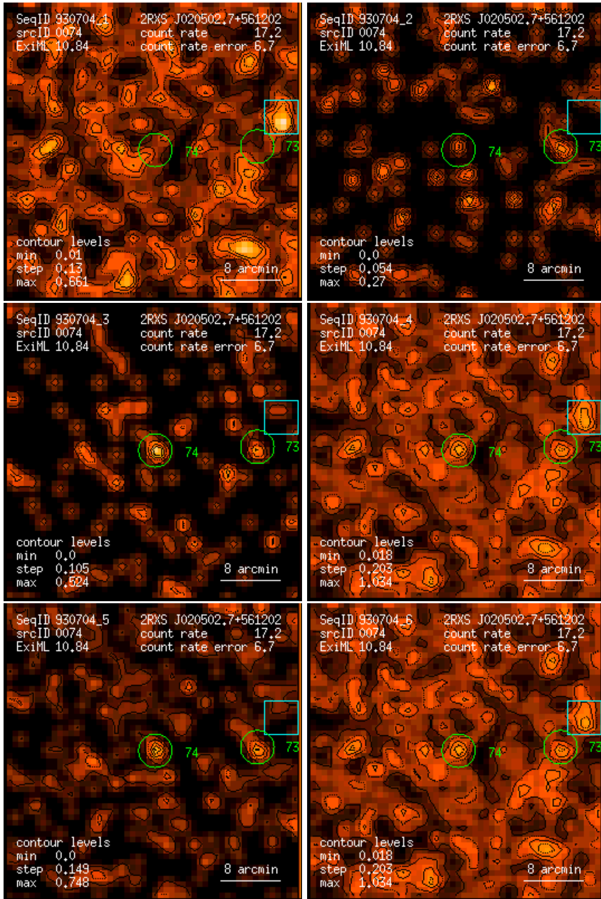
Figure 74: RASS 930704: detection 0074: band rate images, Gaussian filter: (1) PSPC channels 11 – 41, (2) 52 – 90, (3) 91 – 201, (4) 11 – 235, (5) 52 – 201, (6) 11 – 201. Broad band rates in counts/ks. Band rate contour levels in counts/ks/arcmin 2 .
