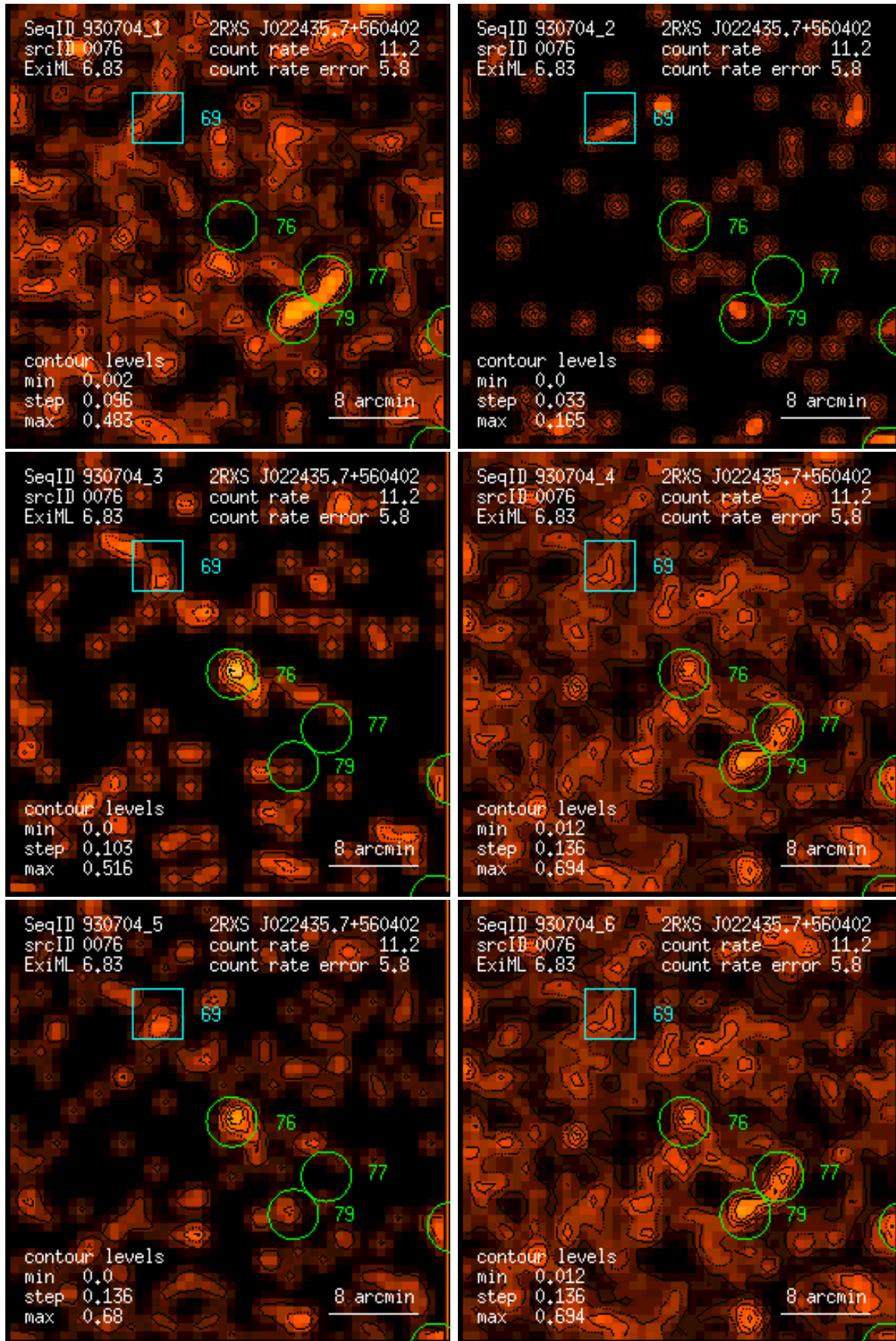
Figure 76: RASS 930704: detection 0076: band rate images, Gaussian filter: (1) PSPC channels 11 – 41, (2) 52 – 90, (3) 91 – 201, (4) 11 – 235, (5) 52 – 201, (6) 11 – 201. Broad band rates in counts/ks. Band rate contour levels in counts/ks/arcmin 2 .
