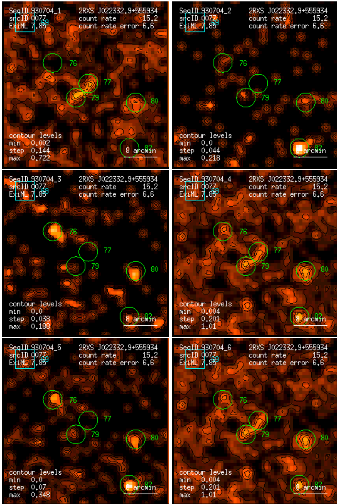
Figure 77: RASS 930704: detection 0077: band rate images, Gaussian filter: (1) PSPC channels 11 – 41, (2) 52 – 90, (3) 91 – 201, (4) 11 – 235, (5) 52 – 201, (6) 11 – 201. Broad band rates in counts/ks. Band rate contour levels in counts/ks/arcmin 2 .
