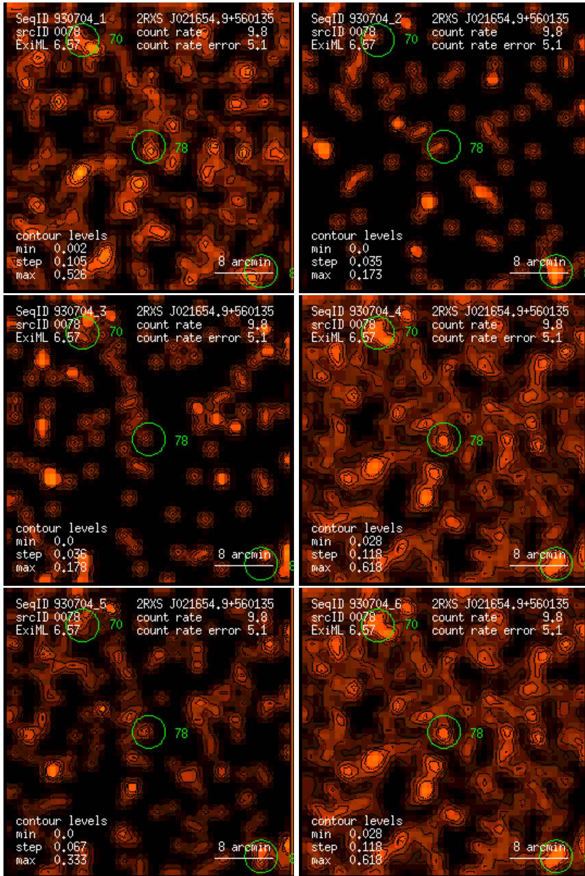
Figure 78: RASS 930704: detection 0078: band rate images, Gaussian filter: (1) PSPC channels 11 – 41, (2) 52 – 90, (3) 91 – 201, (4) 11 – 235, (5) 52 – 201, (6) 11 – 201. Broad band rates in counts/ks. Band rate contour levels in counts/ks/arcmin 2 .
