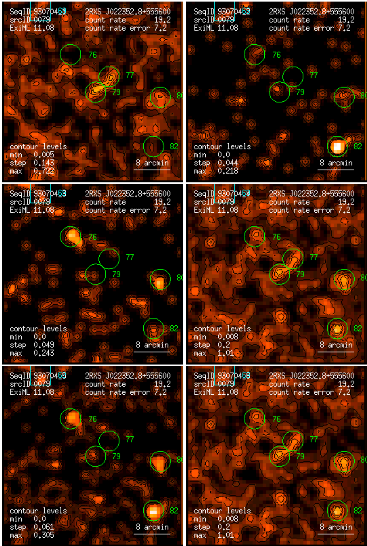
Figure 79: RASS 930704: detection 0079: band rate images, Gaussian filter: (1) PSPC channels 11 – 41, (2) 52 – 90, (3) 91 – 201, (4) 11 – 235, (5) 52 – 201, (6) 11 – 201. Broad band rates in counts/ks. Band rate contour levels in counts/ks/arcmin 2 .
