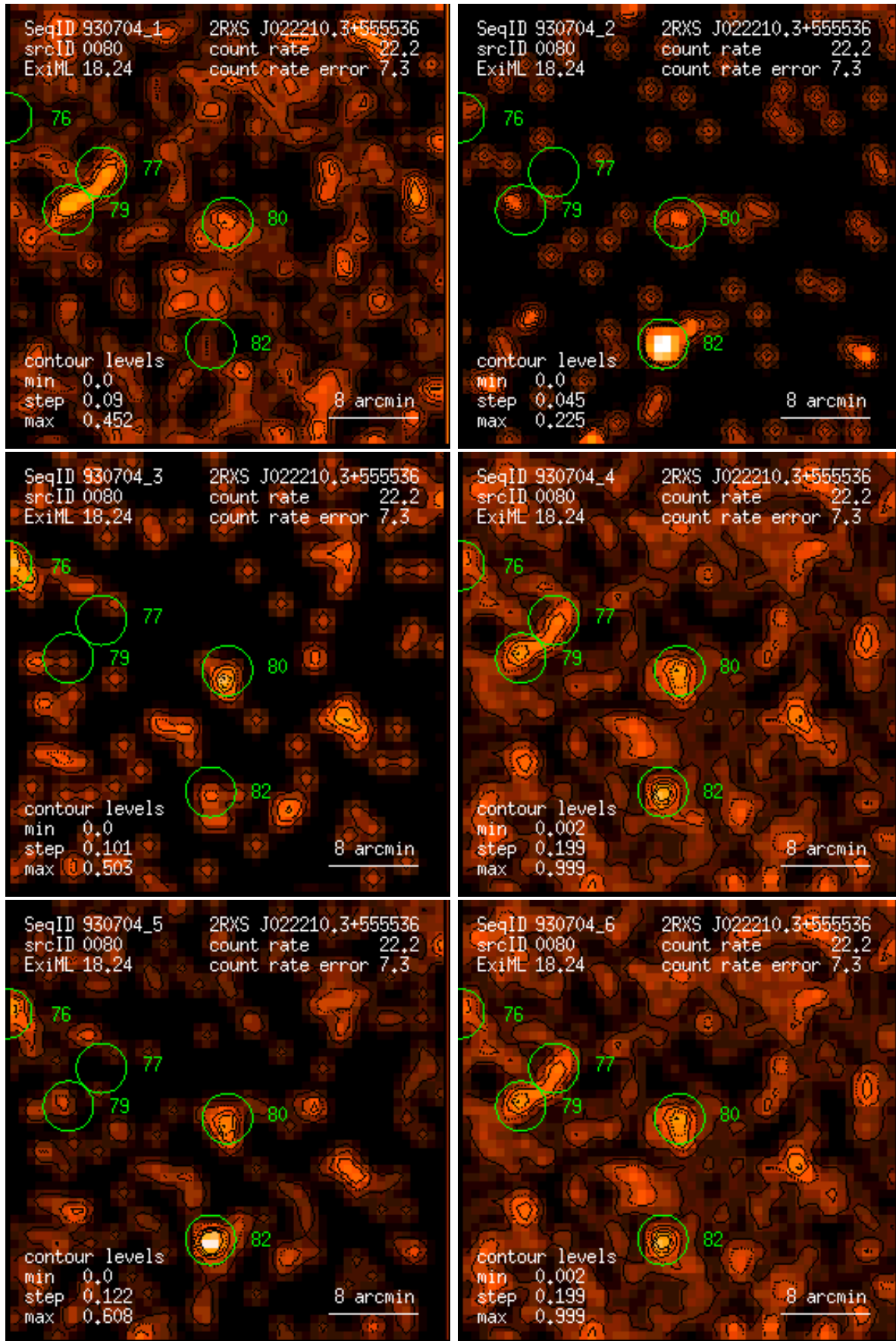
Figure 80: RASS 930704: detection 0080: band rate images, Gaussian filter: (1) PSPC channels 11 – 41, (2) 52 – 90, (3) 91 – 201, (4) 11 – 235, (5) 52 – 201, (6) 11 – 201. Broad band rates in counts/ks. Band rate contour levels in counts/ks/arcmin 2 .
