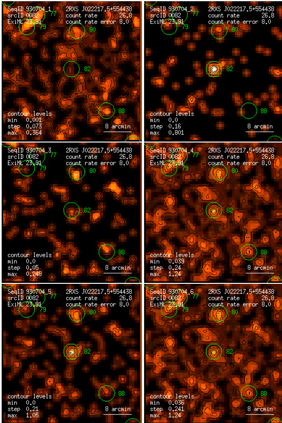
Figure 82: RASS 930704: detection 0082: band rate images, Gaussian filter: (1) PSPC channels 11 – 41, (2) 52 – 90, (3) 91 – 201, (4) 11 – 235, (5) 52 – 201, (6) 11 – 201. Broad band rates in counts/ks. Band rate contour levels in counts/ks/arcmin 2 .
