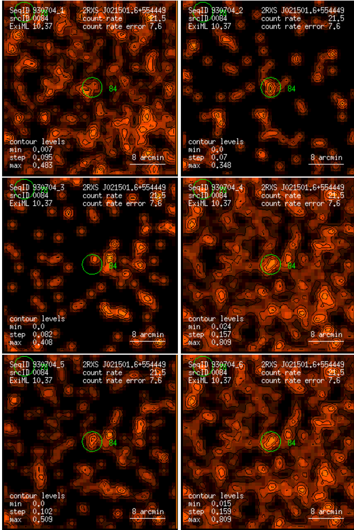
Figure 84: RASS 930704: detection 0084: band rate images, Gaussian filter: (1) PSPC channels 11 – 41, (2) 52 – 90, (3) 91 – 201, (4) 11 – 235, (5) 52 – 201, (6) 11 – 201. Broad band rates in counts/ks. Band rate contour levels in counts/ks/arcmin 2 .
