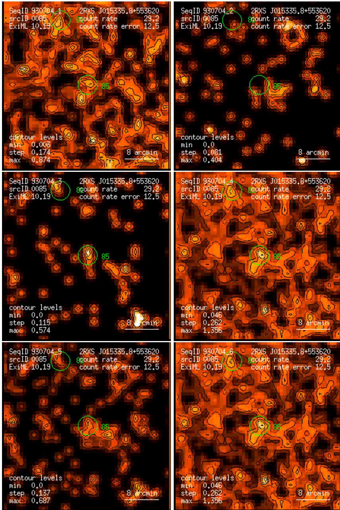
Figure 85: RASS 930704: detection 0085: band rate images, Gaussian filter: (1) PSPC channels 11 – 41, (2) 52 – 90, (3) 91 – 201, (4) 11 – 235, (5) 52 – 201, (6) 11 – 201. Broad band rates in counts/ks. Band rate contour levels in counts/ks/arcmin 2 .
