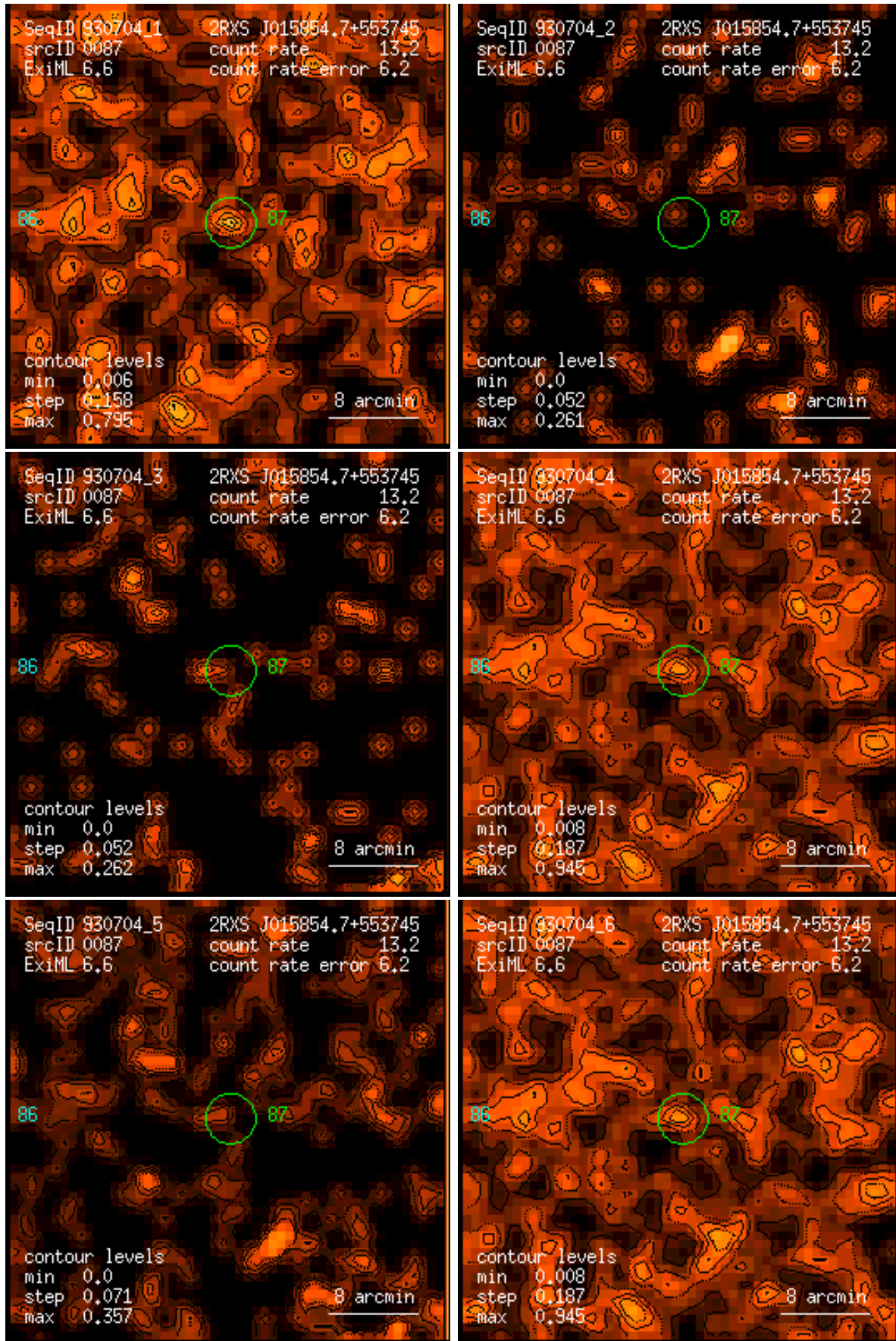
Figure 87: RASS 930704: detection 0087: band rate images, Gaussian filter: (1) PSPC channels 11 – 41, (2) 52 – 90, (3) 91 – 201, (4) 11 – 235, (5) 52 – 201, (6) 11 – 201. Broad band rates in counts/ks. Band rate contour levels in counts/ks/arcmin 2 .
