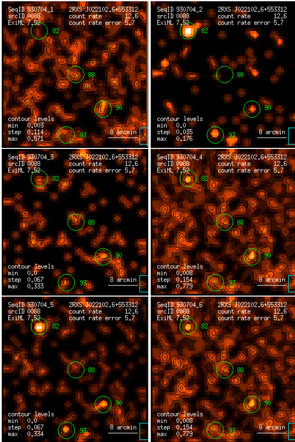
Figure 88: RASS 930704: detection 0088: band rate images, Gaussian filter: (1) PSPC channels 11 – 41, (2) 52 – 90, (3) 91 – 201, (4) 11 – 235, (5) 52 – 201, (6) 11 – 201. Broad band rates in counts/ks. Band rate contour levels in counts/ks/arcmin 2 .
