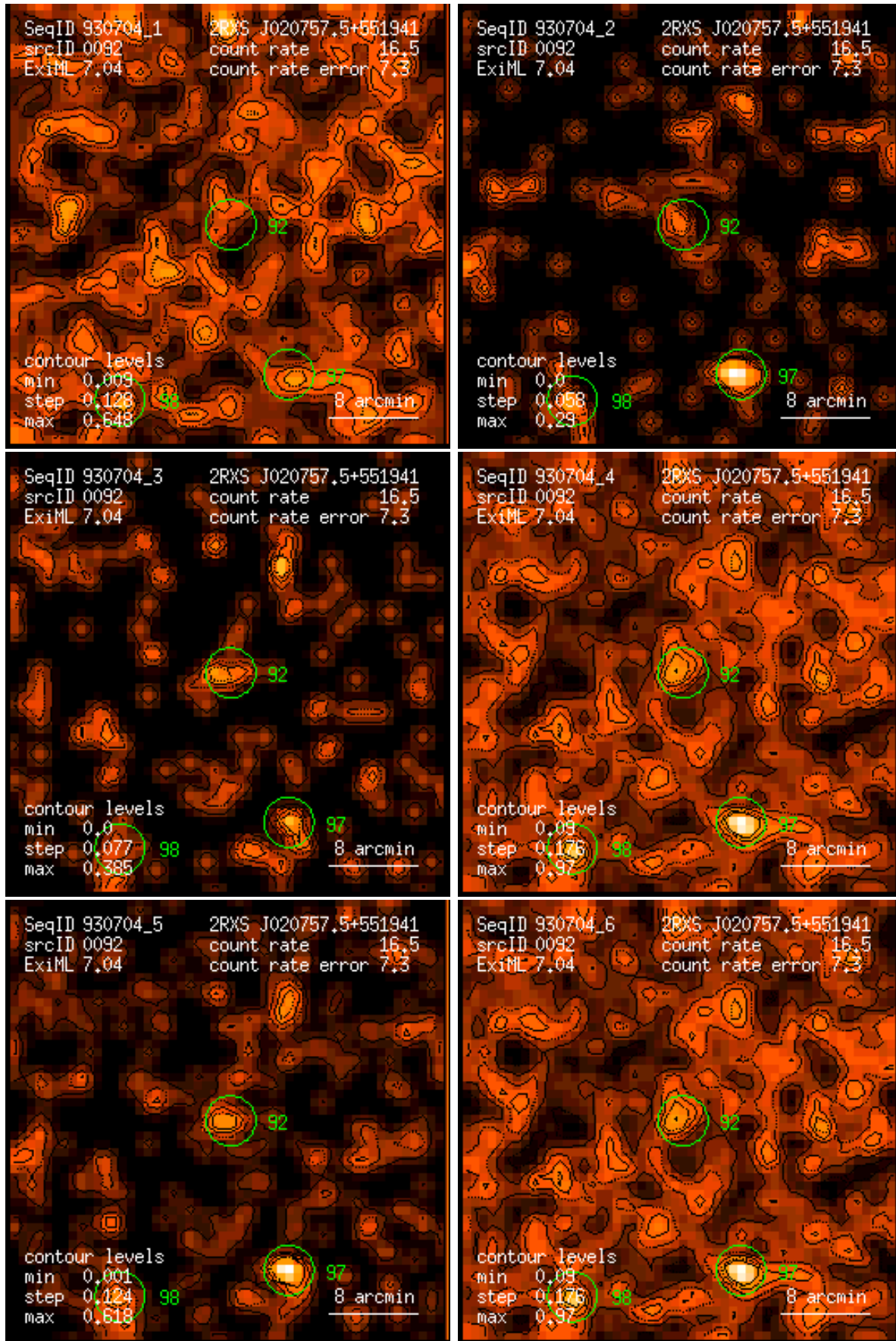
Figure 92: RASS 930704: detection 0092: band rate images, Gaussian filter: (1) PSPC channels 11 – 41, (2) 52 – 90, (3) 91 – 201, (4) 11 – 235, (5) 52 – 201, (6) 11 – 201. Broad band rates in counts/ks. Band rate contour levels in counts/ks/arcmin 2 .
