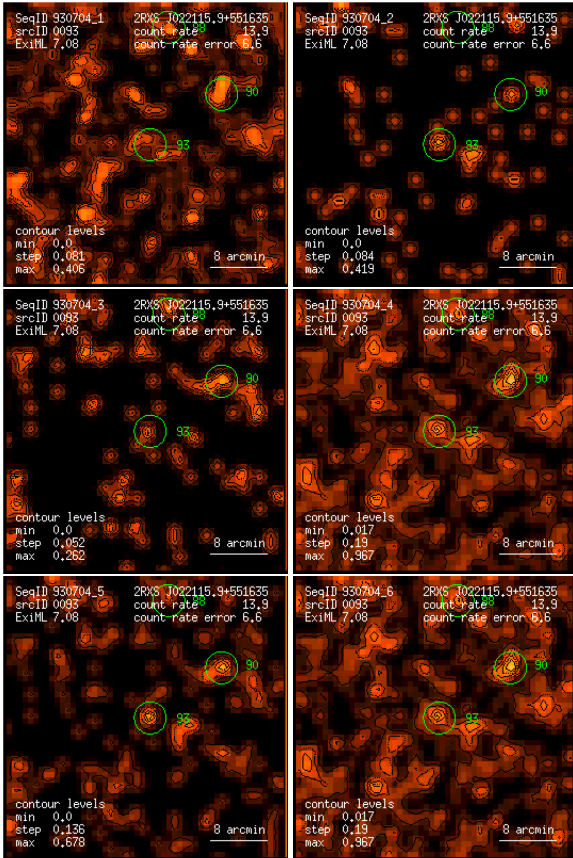
Figure 93: RASS 930704: detection 0093: band rate images, Gaussian filter: (1) PSPC channels 11 – 41, (2) 52 – 90, (3) 91 – 201, (4) 11 – 235, (5) 52 – 201, (6) 11 – 201. Broad band rates in counts/ks. Band rate contour levels in counts/ks/arcmin 2 .
