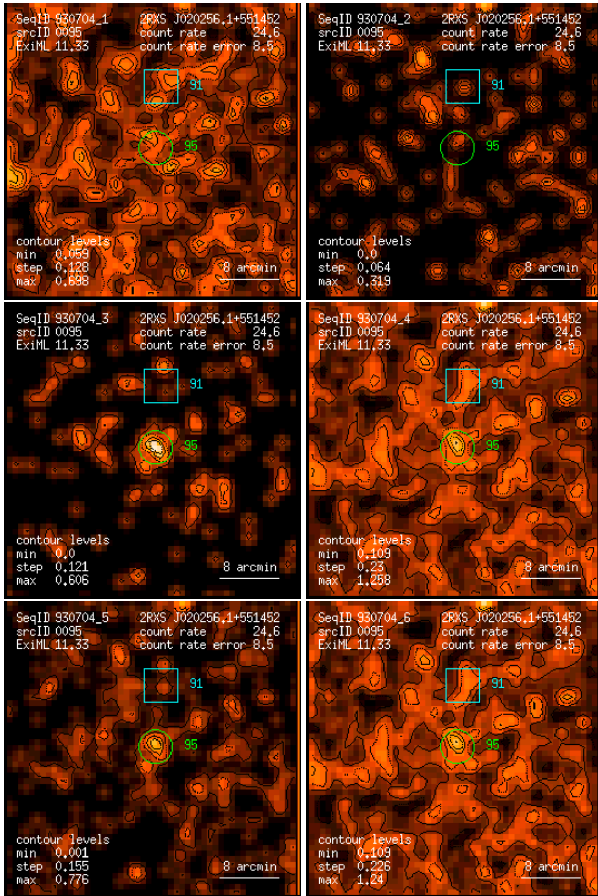
Figure 95: RASS 930704: detection 0095: band rate images, Gaussian filter: (1) PSPC channels 11 – 41, (2) 52 – 90, (3) 91 – 201, (4) 11 – 235, (5) 52 – 201, (6) 11 – 201. Broad band rates in counts/ks. Band rate contour levels in counts/ks/arcmin 2 .
