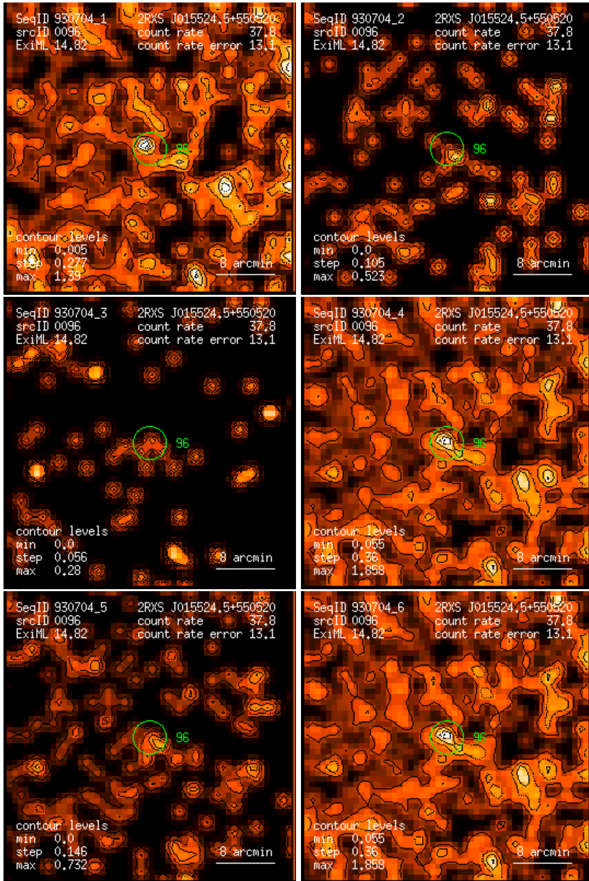
Figure 96: RASS 930704: detection 0096: band rate images, Gaussian filter: (1) PSPC channels 11 – 41, (2) 52 – 90, (3) 91 – 201, (4) 11 – 235, (5) 52 – 201, (6) 11 – 201. Broad band rates in counts/ks. Band rate contour levels in counts/ks/arcmin 2 .
