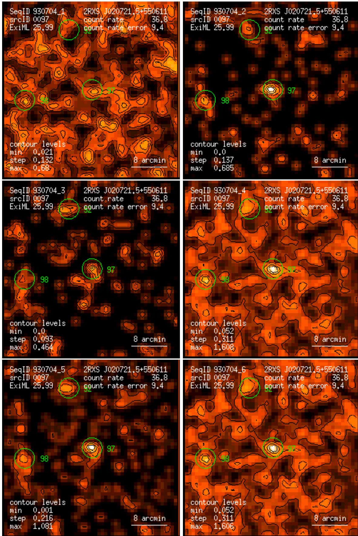
Figure 97: RASS 930704: detection 0097: band rate images, Gaussian filter: (1) PSPC channels 11 – 41, (2) 52 – 90, (3) 91 – 201, (4) 11 – 235, (5) 52 – 201, (6) 11 – 201. Broad band rates in counts/ks. Band rate contour levels in counts/ks/arcmin 2 .
