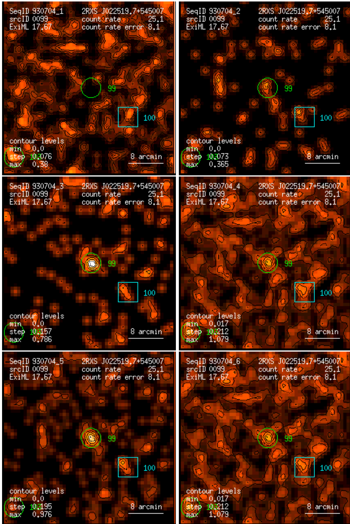
Figure 99: RASS 930704: detection 0099: band rate images, Gaussian filter: (1) PSPC channels 11 – 41, (2) 52 – 90, (3) 91 – 201, (4) 11 – 235, (5) 52 – 201, (6) 11 – 201. Broad band rates in counts/ks. Band rate contour levels in counts/ks/arcmin 2 .
