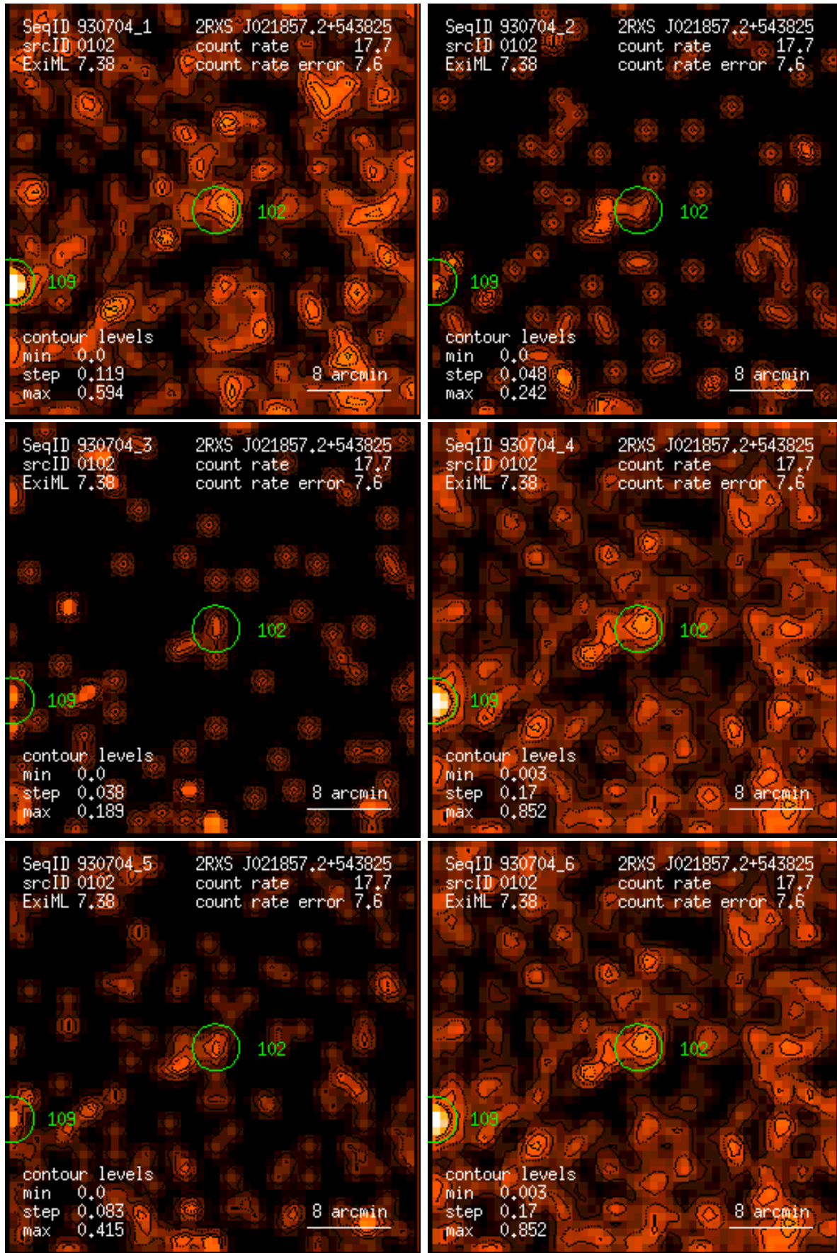
Figure 102: RASS 930704: detection 0102: band rate images, Gaussian filter: (1) PSPC channels 11 – 41, (2) 52 – 90, (3) 91 – 201, (4) 11 – 235, (5) 52 – 201, (6) 11 – 201. Broad band rates in counts/ks. Band rate contour levels in counts/ks/arcmin 2 .
