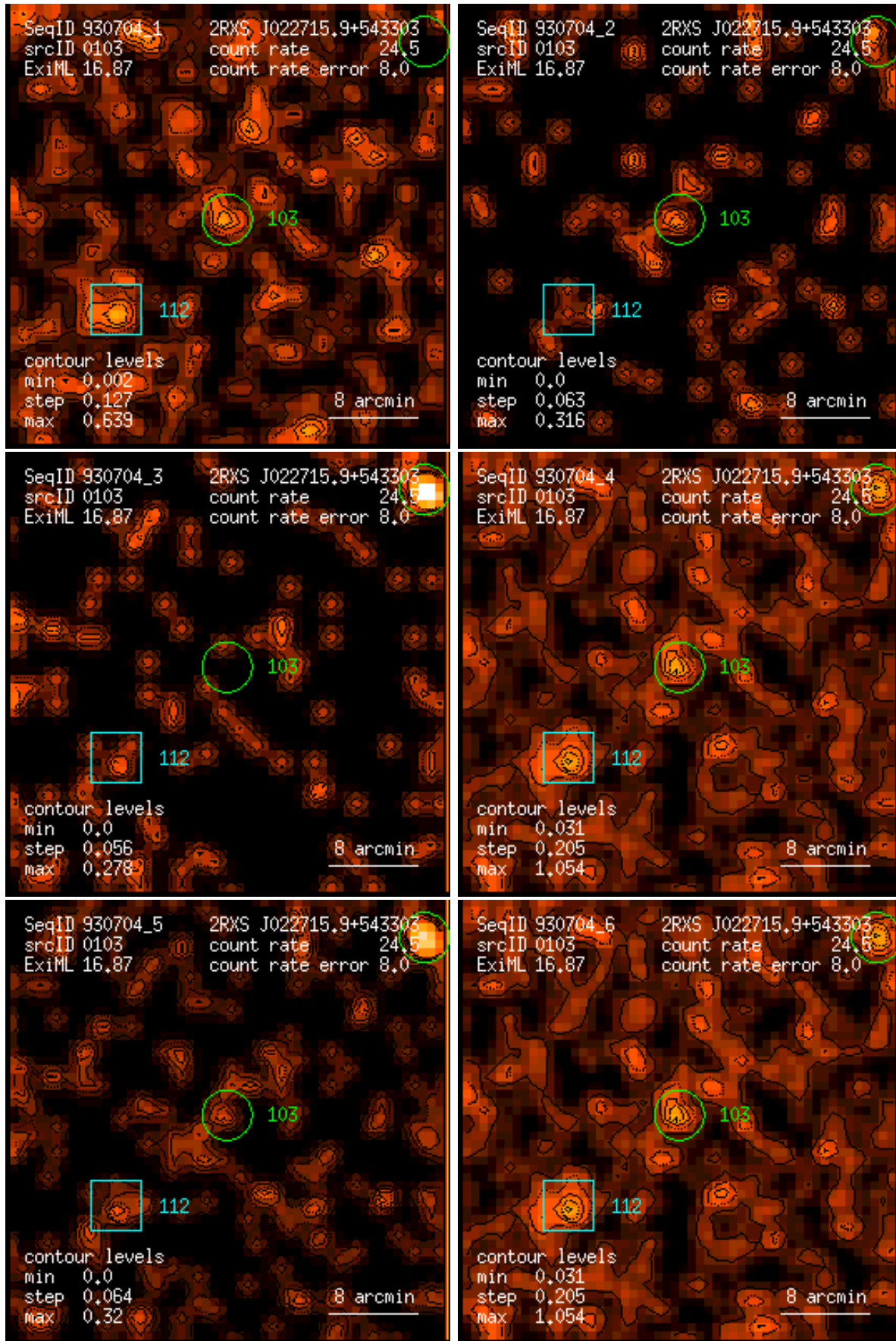
Figure 103: RASS 930704: detection 0103: band rate images, Gaussian filter: (1) PSPC channels 11 – 41, (2) 52 – 90, (3) 91 – 201, (4) 11 – 235, (5) 52 – 201, (6) 11 – 201. Broad band rates in counts/ks. Band rate contour levels in counts/ks/arcmin 2 .
