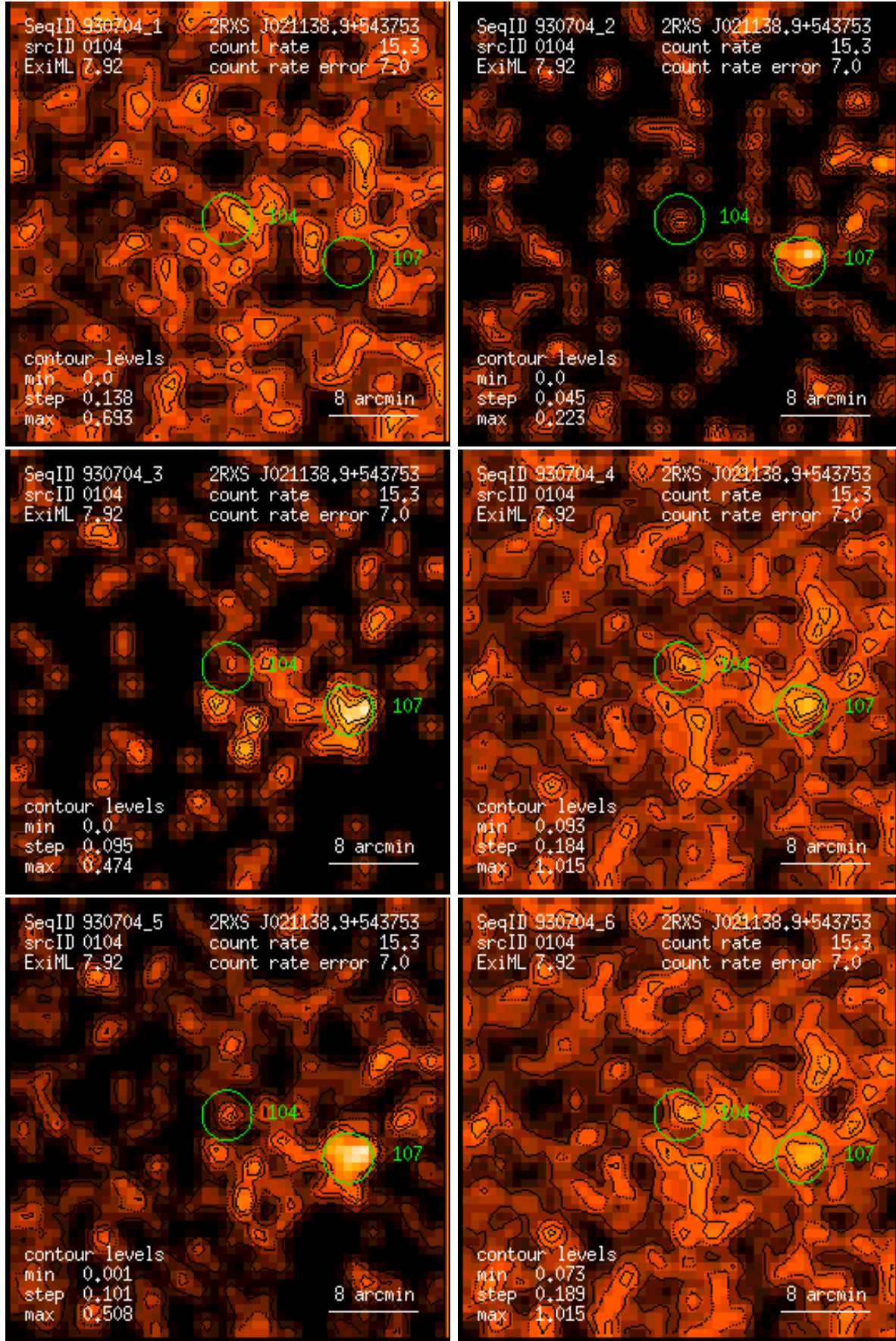
Figure 104: RASS 930704: detection 0104: band rate images, Gaussian filter: (1) PSPC channels 11 – 41, (2) 52 – 90, (3) 91 – 201, (4) 11 – 235, (5) 52 – 201, (6) 11 – 201. Broad band rates in counts/ks. Band rate contour levels in counts/ks/arcmin 2 .
