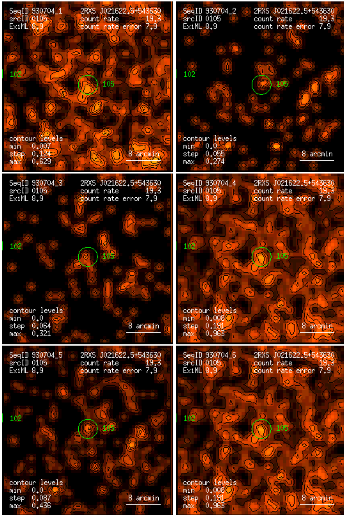
Figure 105: RASS 930704: detection 0105: band rate images, Gaussian filter: (1) PSPC channels 11 – 41, (2) 52 – 90, (3) 91 – 201, (4) 11 – 235, (5) 52 – 201, (6) 11 – 201. Broad band rates in counts/ks. Band rate contour levels in counts/ks/arcmin 2 .
