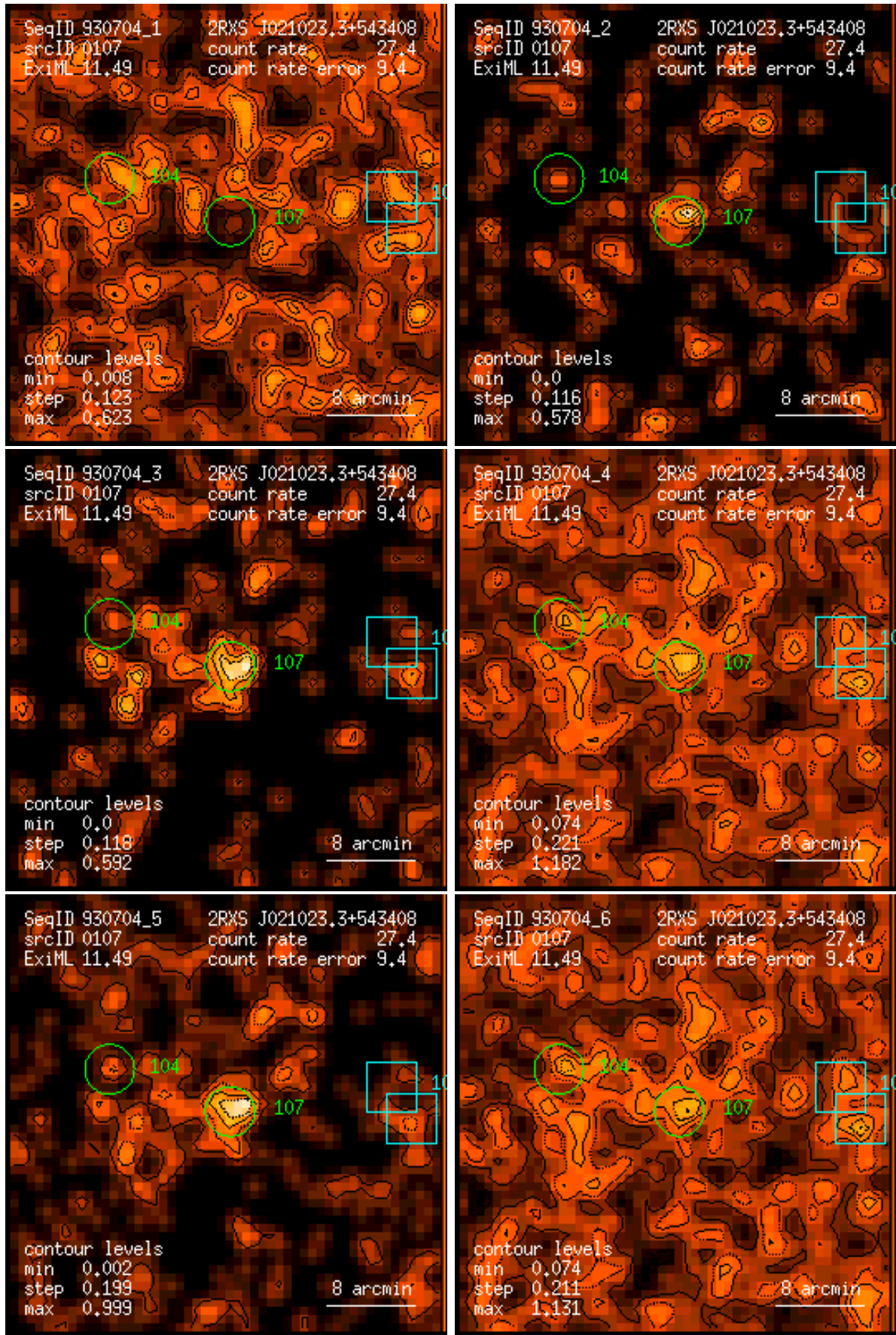
Figure 107: RASS 930704: detection 0107: band rate images, Gaussian filter: (1) PSPC channels 11 – 41, (2) 52 – 90, (3) 91 – 201, (4) 11 – 235, (5) 52 – 201, (6) 11 – 201. Broad band rates in counts/ks. Band rate contour levels in counts/ks/arcmin 2 .
