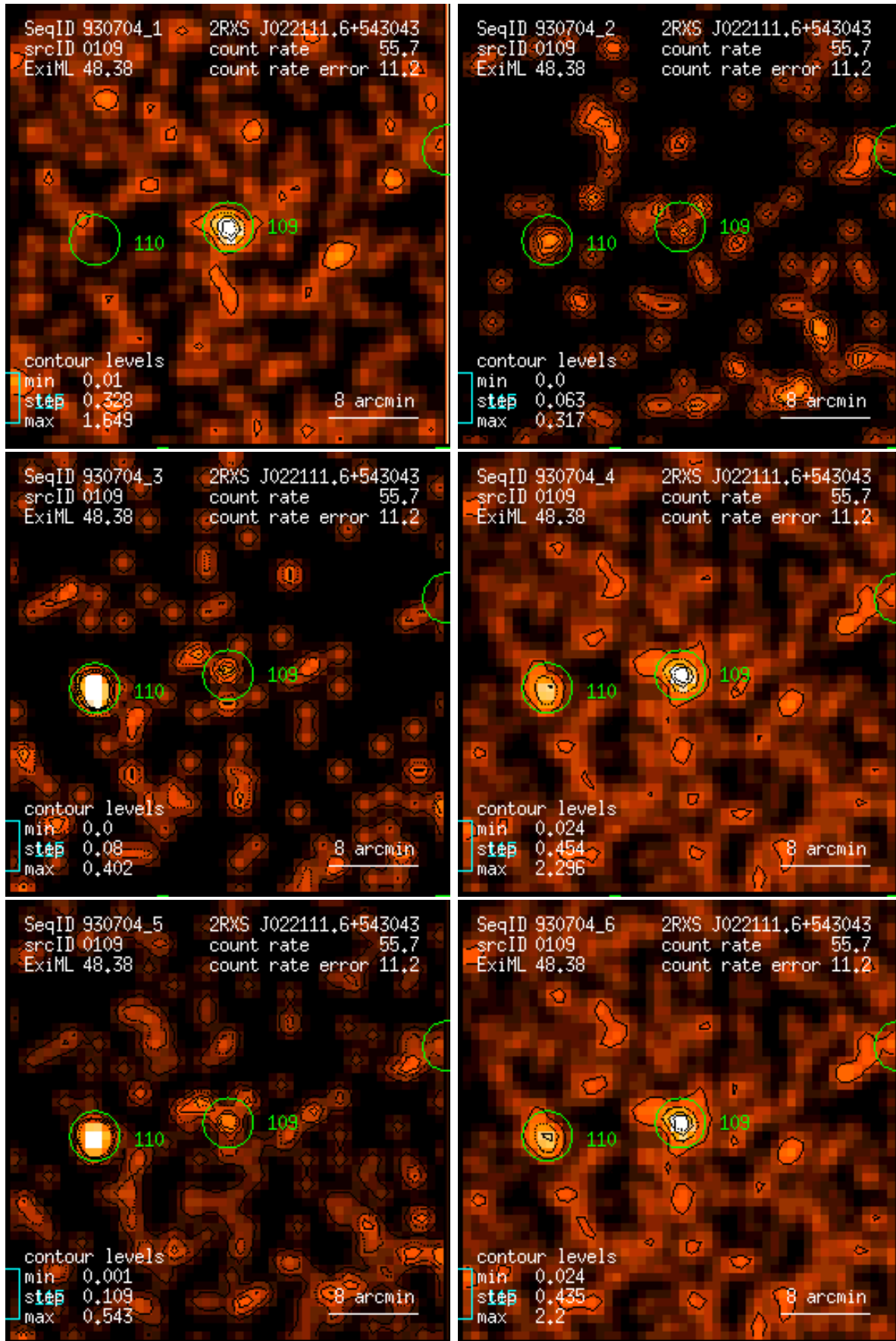
Figure 109: RASS 930704: detection 0109: band rate images, Gaussian filter: (1) PSPC channels 11 – 41, (2) 52 – 90, (3) 91 – 201, (4) 11 – 235, (5) 52 – 201, (6) 11 – 201. Broad band rates in counts/ks. Band rate contour levels in counts/ks/arcmin 2 .
