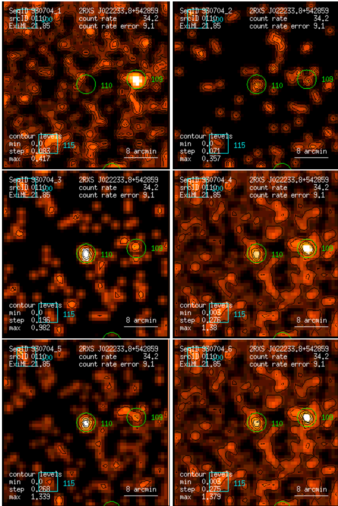
Figure 110: RASS 930704: detection 0110: band rate images, Gaussian filter: (1) PSPC channels 11 – 41, (2) 52 – 90, (3) 91 – 201, (4) 11 – 235, (5) 52 – 201, (6) 11 – 201. Broad band rates in counts/ks. Band rate contour levels in counts/ks/arcmin 2 .
