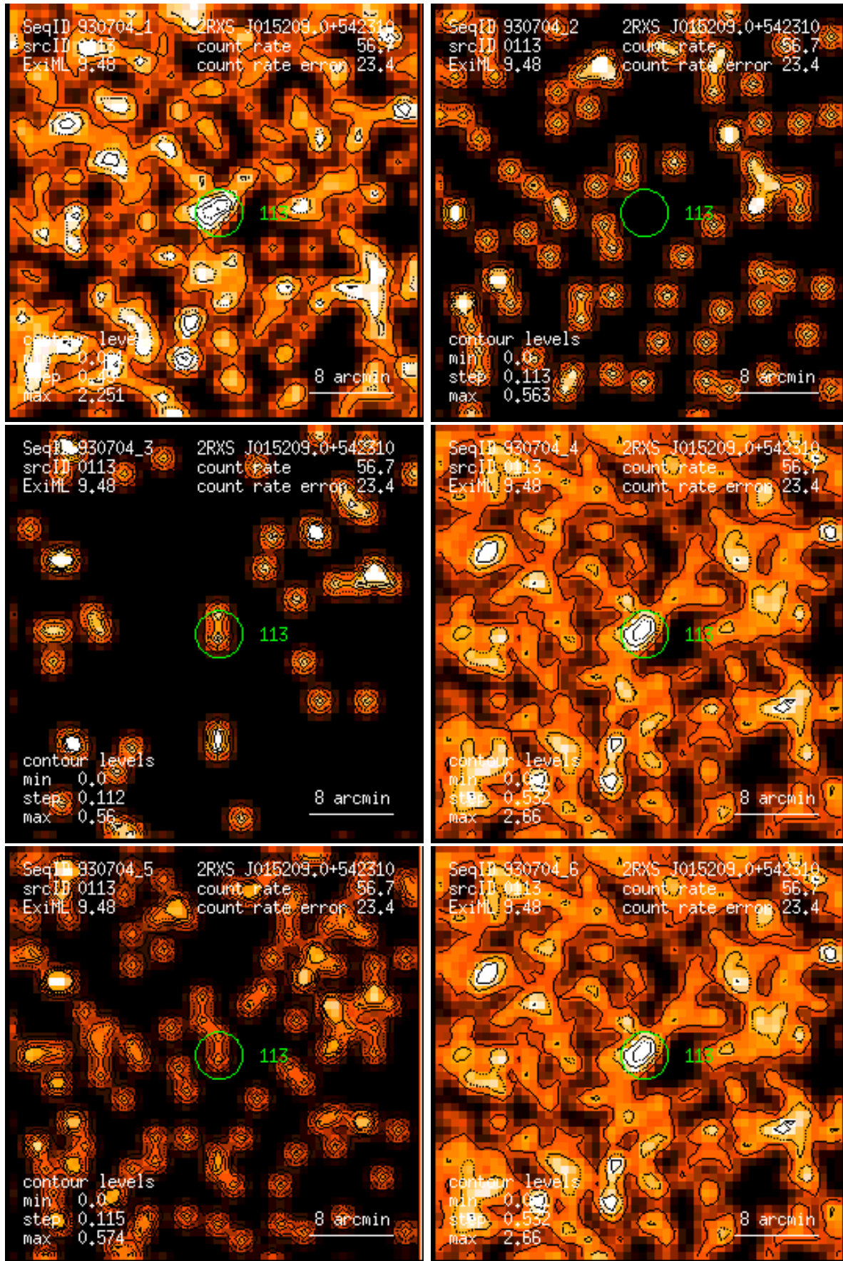
Figure 113: RASS 930704: detection 0113: band rate images, Gaussian filter: (1) PSPC channels 11 – 41, (2) 52 – 90, (3) 91 – 201, (4) 11 – 235, (5) 52 – 201, (6) 11 – 201. Broad band rates in counts/ks. Band rate contour levels in counts/ks/arcmin 2 .
