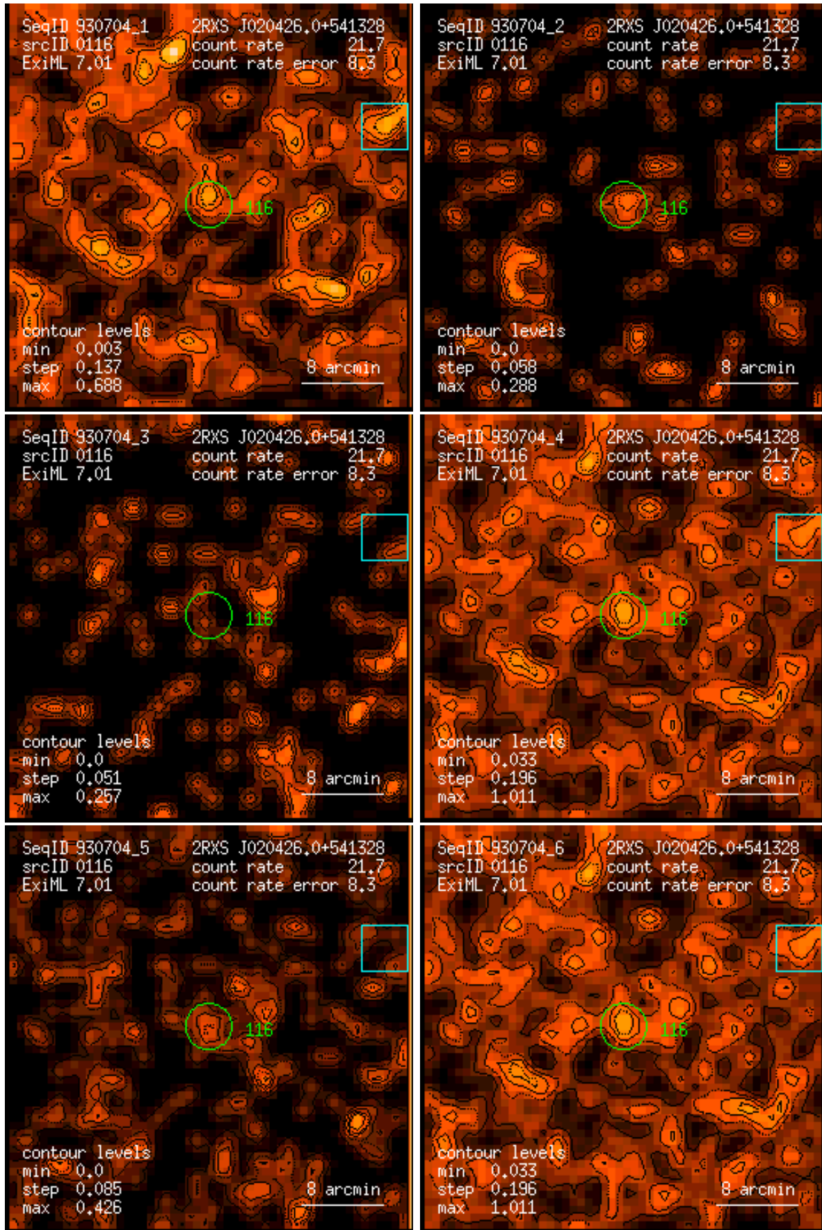
Figure 116: RASS 930704: detection 0116: band rate images, Gaussian filter: (1) PSPC channels 11 – 41, (2) 52 – 90, (3) 91 – 201, (4) 11 – 235, (5) 52 – 201, (6) 11 – 201. Broad band rates in counts/ks. Band rate contour levels in counts/ks/arcmin 2 .
