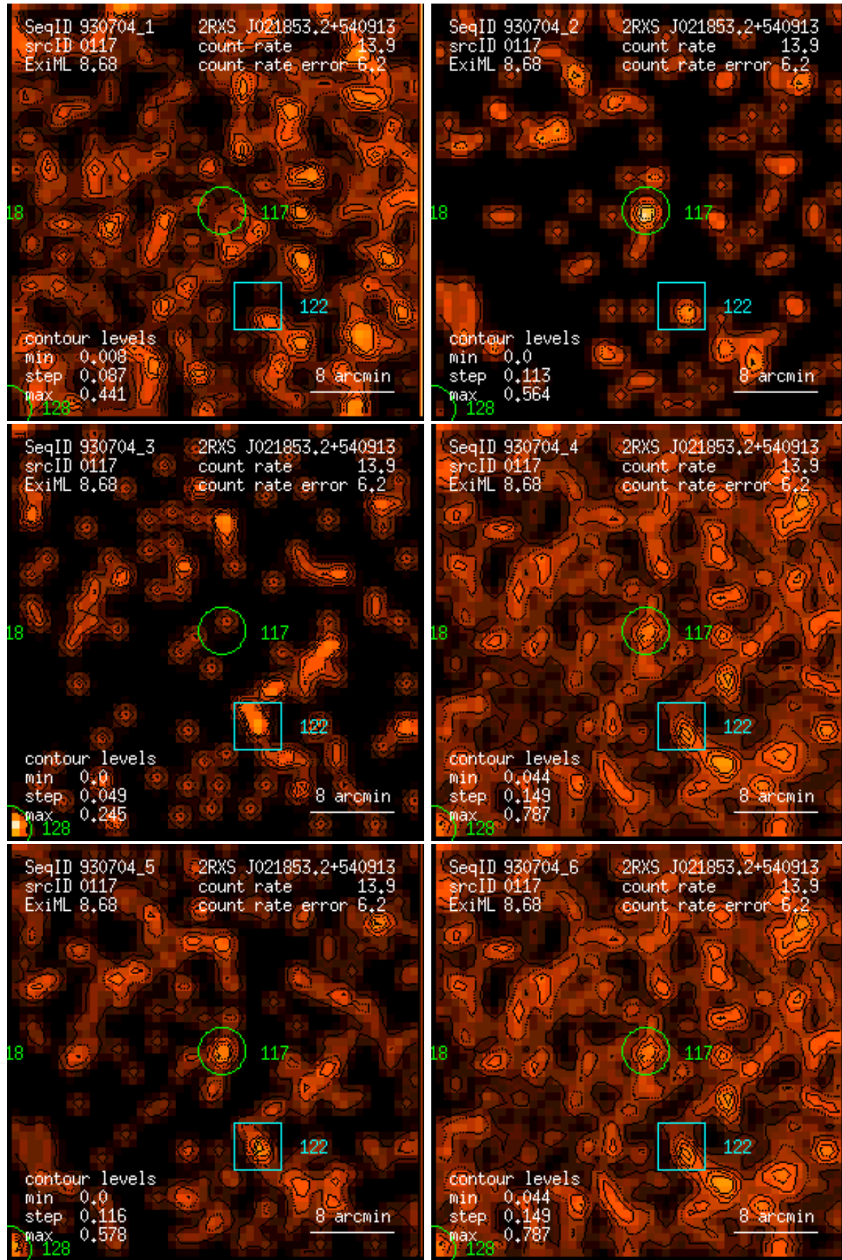
Figure 117: RASS 930704: detection 0117: band rate images, Gaussian filter: (1) PSPC channels 11 – 41, (2) 52 – 90, (3) 91 – 201, (4) 11 – 235, (5) 52 – 201, (6) 11 – 201. Broad band rates in counts/ks. Band rate contour levels in counts/ks/arcmin 2 .
