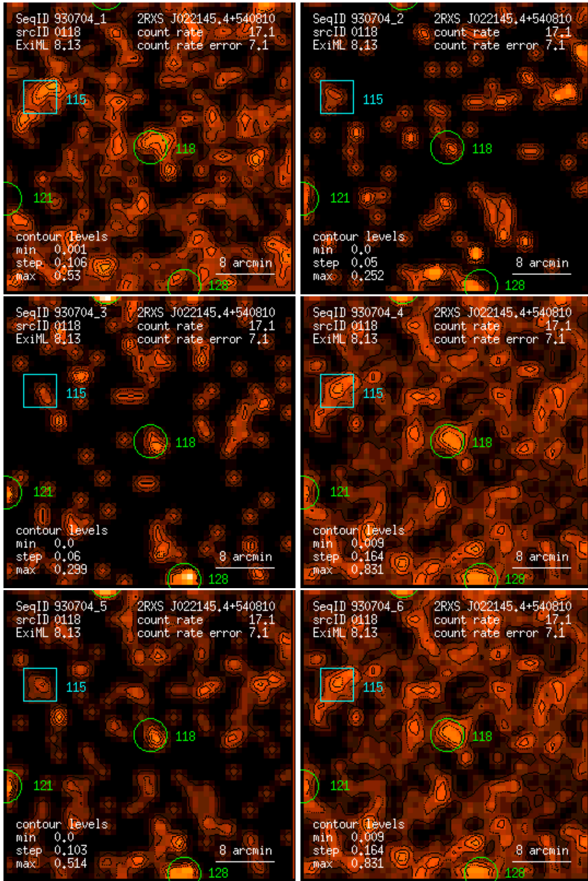
Figure 118: RASS 930704: detection 0118: band rate images, Gaussian filter: (1) PSPC channels 11 – 41, (2) 52 – 90, (3) 91 – 201, (4) 11 – 235, (5) 52 – 201, (6) 11 – 201. Broad band rates in counts/ks. Band rate contour levels in counts/ks/arcmin 2 .
