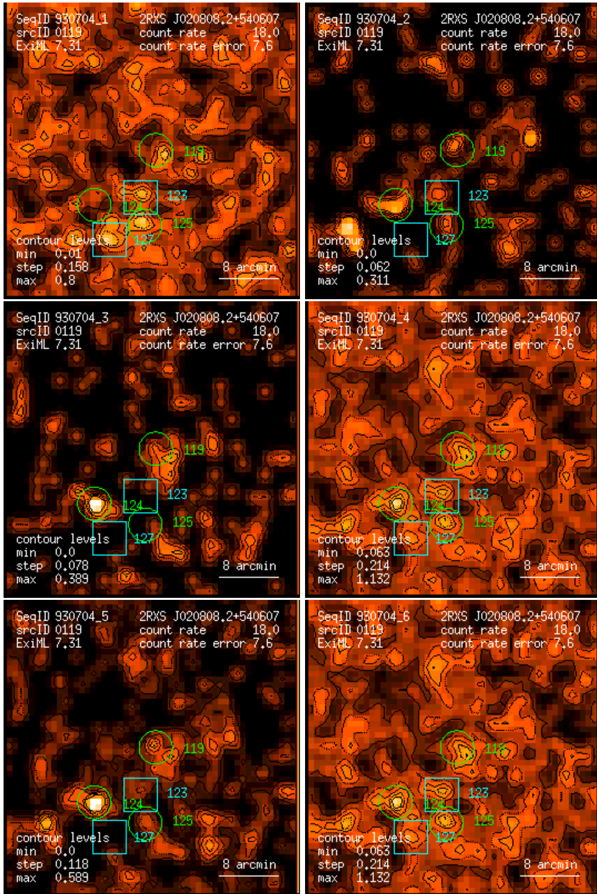
Figure 119: RASS 930704: detection 0119: band rate images, Gaussian filter: (1) PSPC channels 11 – 41, (2) 52 – 90, (3) 91 – 201, (4) 11 – 235, (5) 52 – 201, (6) 11 – 201. Broad band rates in counts/ks. Band rate contour levels in counts/ks/arcmin 2 .
